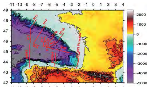
Bathymetry
