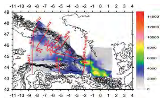
Sediment Thickness
