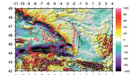
Free Air Gravity
