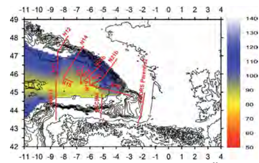
Oceanic Isochrons (Age)
