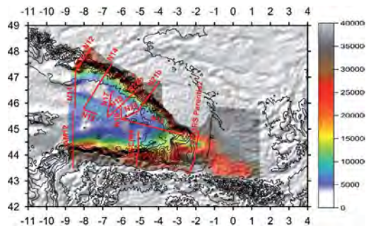
Residual Continental Crust (m)
