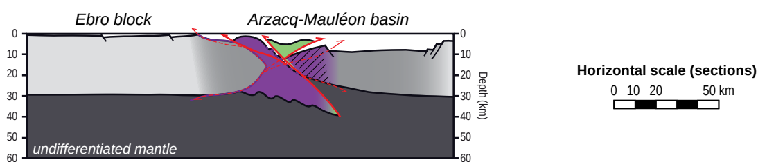
(c) Pyrenean segment
