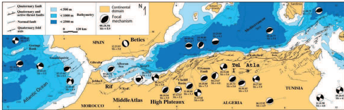
Figure 3: principal fault in North Africa and south European plates. The limitation of the tectonic plates and the principal faults mechanism are shown. Faulcal mechanisms are plotted using Global CMT.
