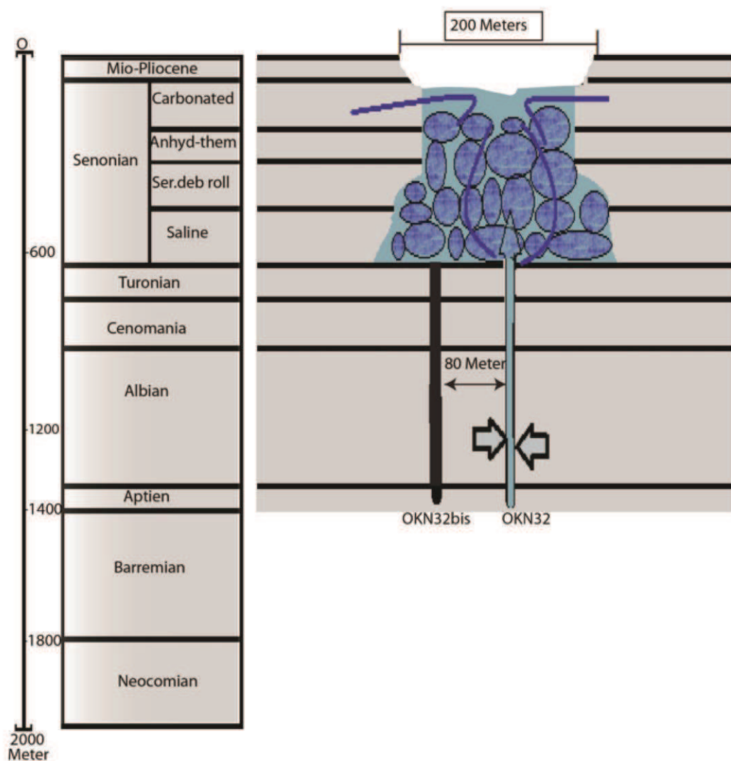
Fig. 4. Oil wells OKN32 and OKN32bis and the stratigraphic log with the schematic illustrated collapse. The Albian hot water that flows within the lower Senonian saline layer is responsible of the well collapse generating a crater with a 200 m diameter.
