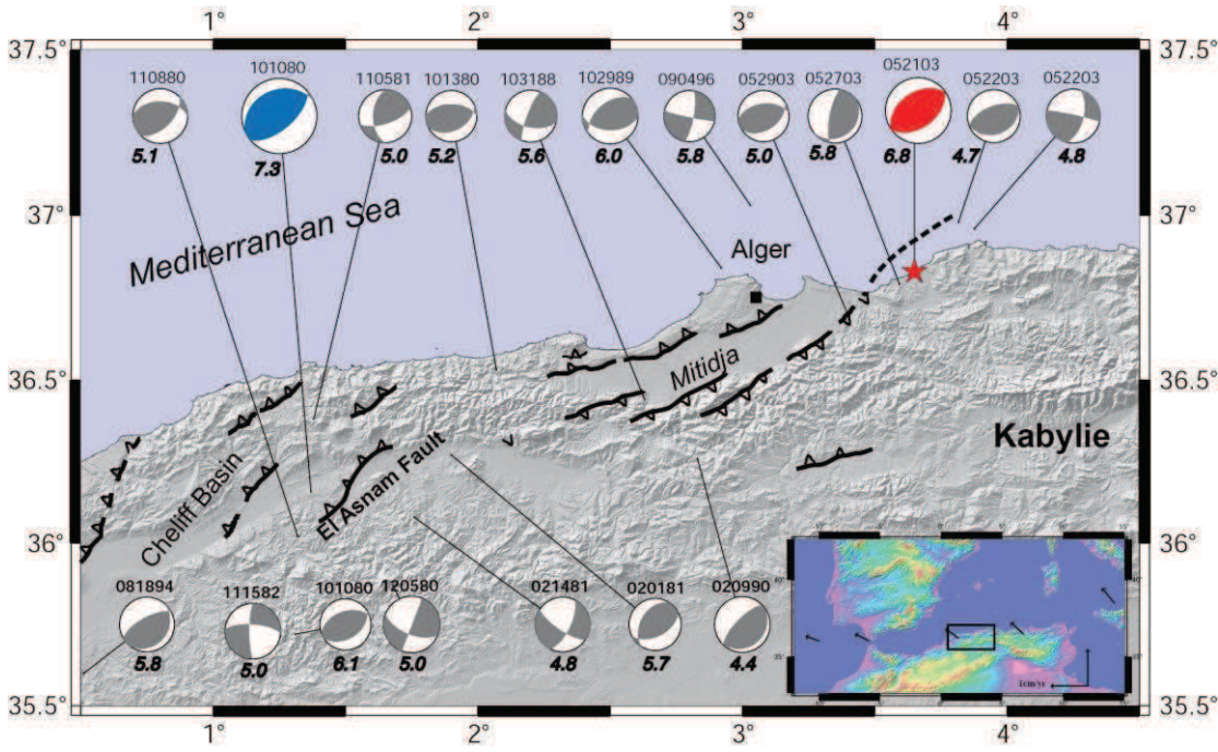
Figure 1: Seismotectonic setting of NW Algeria (Meghraoui, 1988). The El Asnam (Algeria) earthquake of 10/10/1980 ( M_s=7.3 , blue CMT mechanism) occurred in the western Mediterranean, inducing NE-SW and E-W trending, 36-km-long of coseismic reverse faulting visible at the surface (Philip et Meghraoui, 1983). The red mechanism is the 2003 Zemmouri earthquake.
