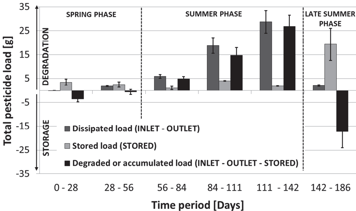
Figure III. 8 Monthly pesticide mass budget emphasizing pesticide storage vs. degradation in the stormwater wetland (Rouffach, Alsace, France). The dissipated pesticide load (INLET load – OUTLET load) refer to the load stored (STORED load) or degraded (INLET load – OUTLET load – STORED load > 0) in the wetland, whereas the accumulated load (INLET load – OUTLET load – STORED load < 0) is the load accumulated in the wetland from one period to the other. The error bars correspond to the analytical uncertainty and, errors were calculated via error propagation, incorporating analytical uncertainties of individual pesticide concentration measurements and the uncertainty of compartmental (bio)mass measurements.
