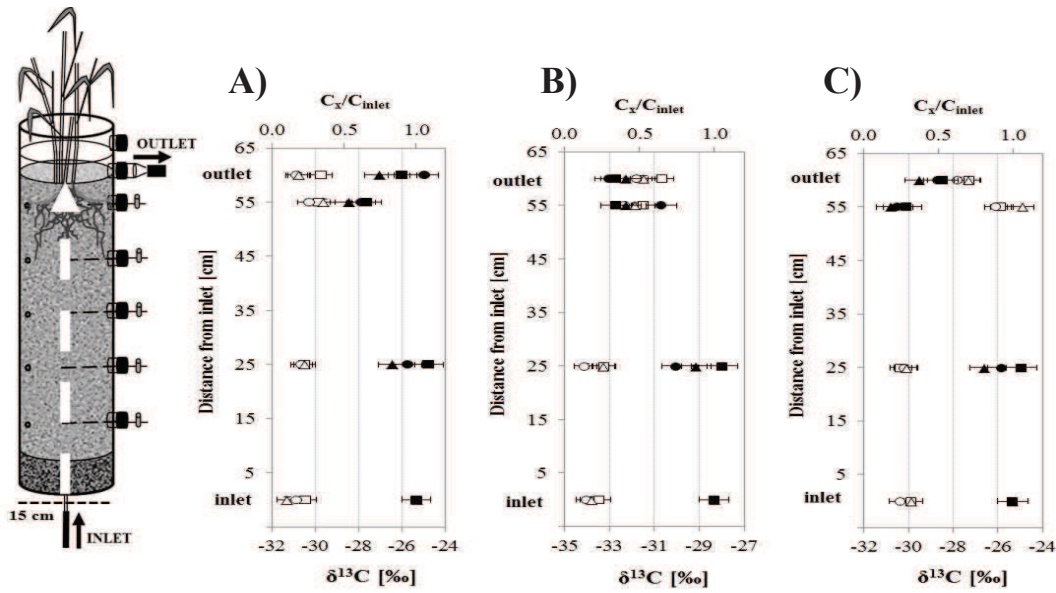
Figure V- 6 Carbon isotope composition represented in \delta^{13}C notation (open symbols) and ratio of concentration at a given point (x) to inlet concentration (filled symbols) of metolachlor A)alachlor B) and acetochlor C) inside lab-scale wetlands on day 42 (squares), day 70 (circles) and day 98 (triangles). Arrows indicate the direction of water flow. Error bars indicate uncertainty of \delta^{13}C ( \pm 0.5\text{‰} ), and propagated error of C_x/C_{inlet} based on standard deviations of concentrations.
