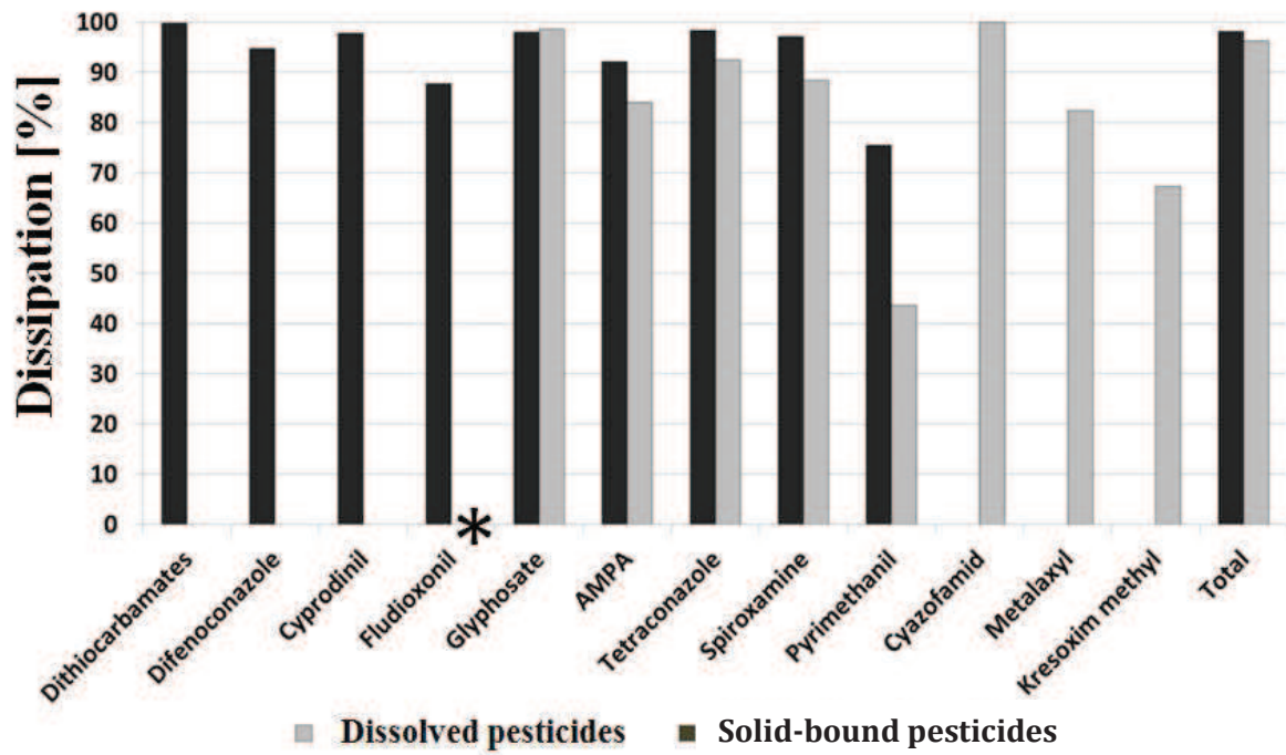
Figure VII- 3. Dissipation rates of dissolved ( < 0.7 \mu\text{m} ) and solid-bound pesticides ( > 0.7 \mu\text{m} ) in the stormwater wetland (Rouffach, Alsace, France) from March 23 rd to September 7 th , 2011.
