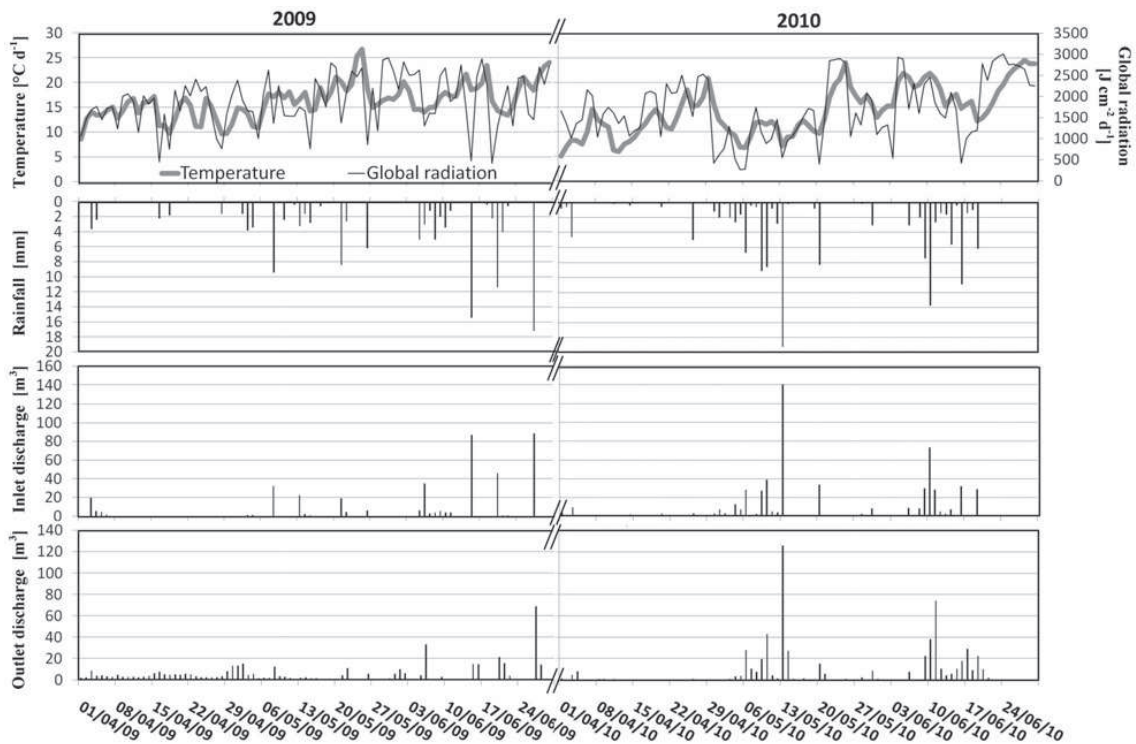
Figure 2. Temporal changes of climatic and hydrological conditions in the vineyard catchment (Rouffach, Haut-Rhin, France) from April 1 to June 30 2009 and 2010.
