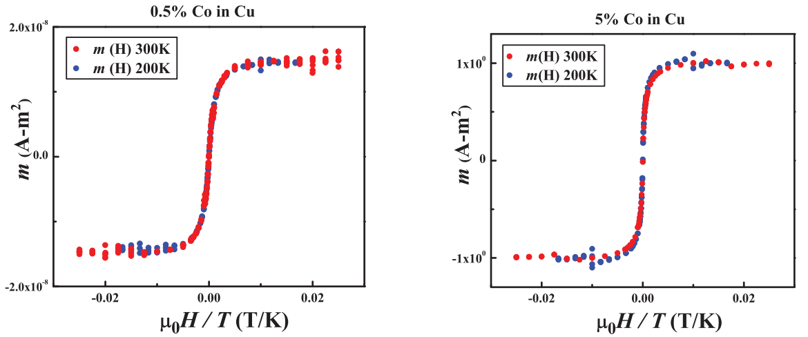
FIG. 62: Magnetization curves as function of H/T at different temperatures for two different concentrations. The curves overlap showing the classical scaling law of superparamagnetism and there are no indications of the influence of the cluster concentration from the magnetization measurement.
