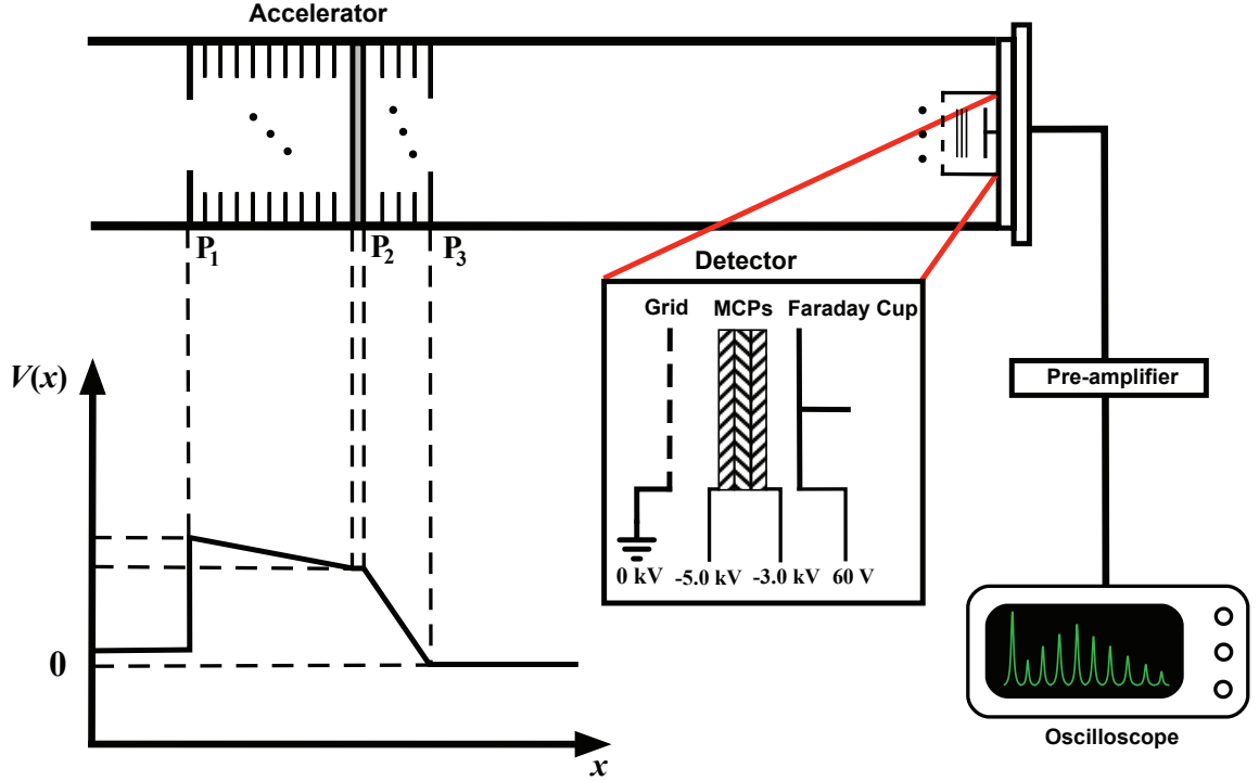
FIG. 6: Schematic illustration of the TOF-MS. The acceleration region consists of two stages separated by a small field free region. At the beginning of each stage a square pulsed electrostatic potential is applied to two plates, the first plate the repeller P_1 and the second plate the extractor P_2 . At the end of the the acceleration region in order to well define the electric field of the exit of the acceleration region a grid P_3 is connected to ground.
