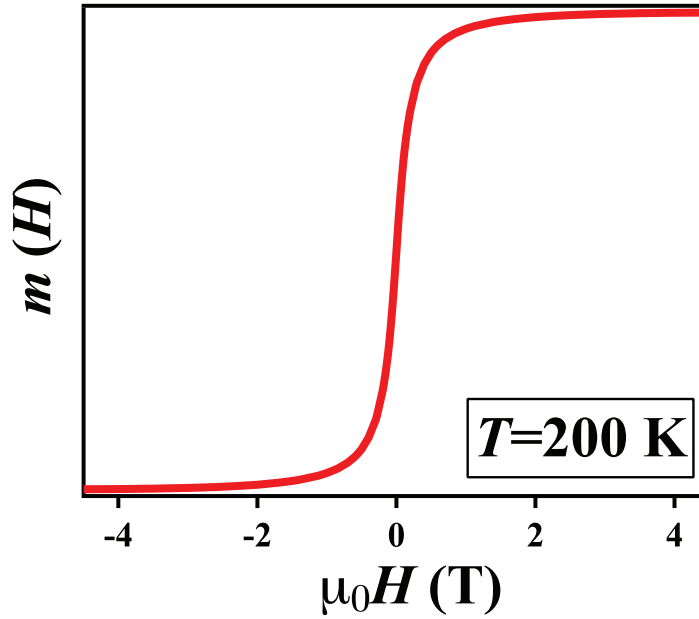
FIG. 23: Simulation of the magnetization as function of the magnetic field described by a Langevin function for an ensemble of particles with 3.5 nm of diameter at a temperature of 200 K.
