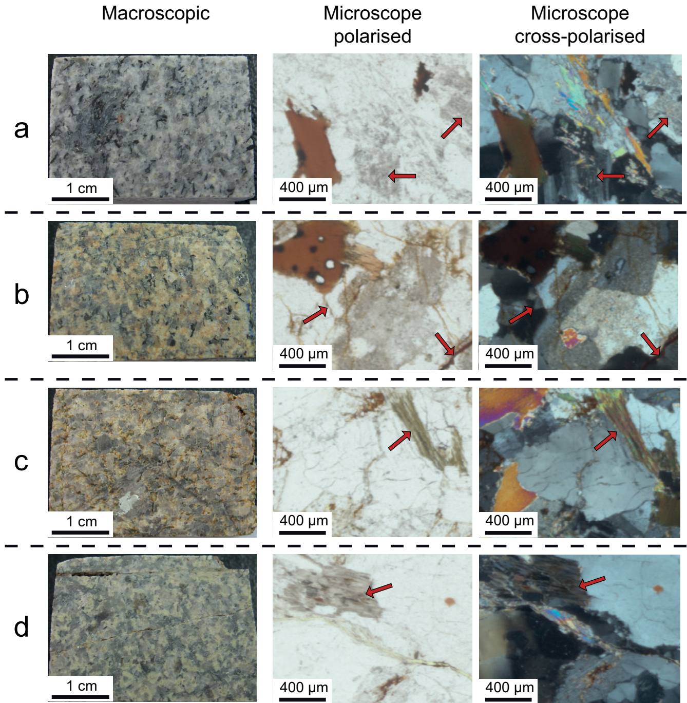
Figure 7. Comparison of sampled granite alteration facies: a - fresh rock: sericitisation of feldspars (sample 11), b - Fe-oxidation: fill of cracks and grain boundaries (sample 3), c - chlorite replacing biotite (sample 7), d - clay minerals replacing biotite (sample 9).
