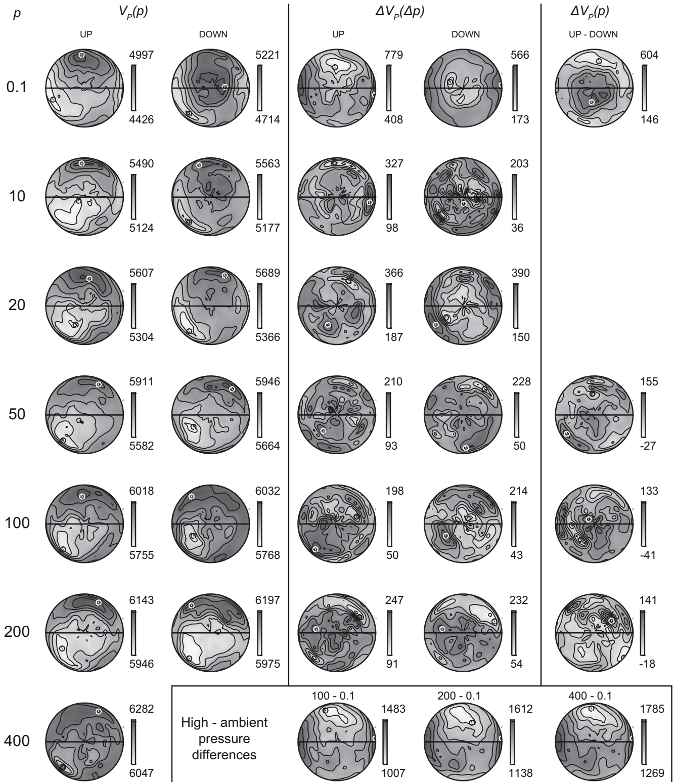
Figure A4 (continued on the following five pages). Results of multidirectional P-wave velocity measurements at high confining pressure. P - confining pressure (MPa), V_p(p) - measured velocity (m s -1 ) at distinct levels of confining pressure, \Delta V_p(\Delta p) - calculated velocity differences (m s -1 ) between the pressure levels, V_p(\Delta p) - calculated velocity differences (m s -1 ) between the pressurisation (UP) and depressurisation (DOWN). In the stereonets the horizontal line shows the orientation of the reference fracture and the solid circles are the directions of maximum (white) and minimum (black) velocities. The maximum and minimum velocities are shown above and below the gray scale, respectively.
