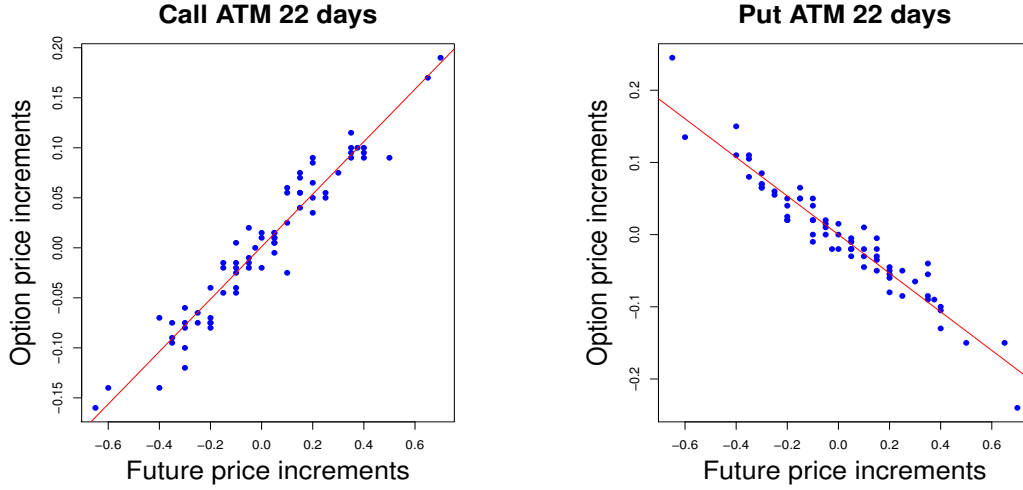
Figure 1.1: Evidence of the linear regression relationship of option price increments and future price increments as observed in the data (here Kospi 200). As expected, the slope is positive for the Call and negative for the Put.
