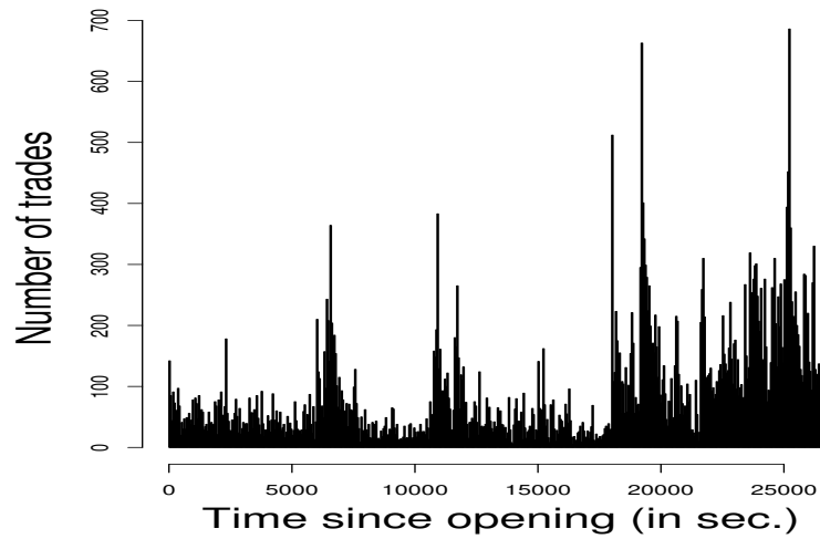
Figure 2.2: Number of trades by time intervals of 1 minute: presence of clusters is graphically apparent. Graph for Eurostoxx futures trades on 2011/03/03.
