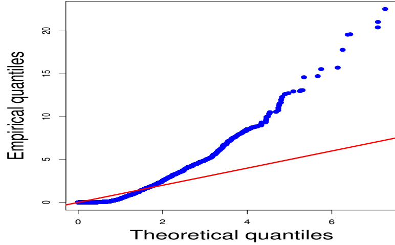
Figure 2.1: QQplot of inter-trade durations against exponential distribution. Inter arrival trade times are clearly not exponential. Graph for Eurostoxx futures trades on 2011/03/03 for the first trading hour.
