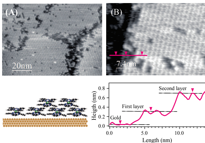
Figure 5.4. STM image of LuPc 2 on Au(111) surface after annealing: (A) 100 nm x 85 nm, V=-0.8V; (B) 37.1 nm x 26.6 nm, V=-0.8V; corresponding line profile is plotted below the image together with a sketch of proposed molecular arrangement. Figure taken from Paper IV.
