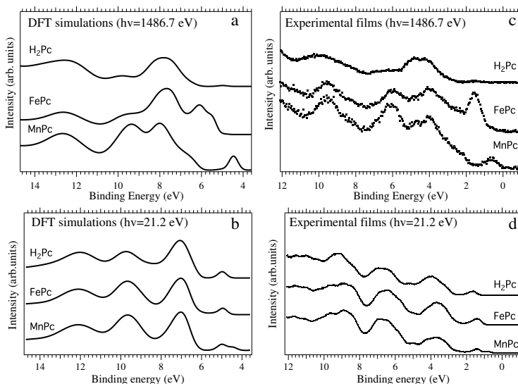
Figure 5.9. a-b: Single molecule DFT simulations of H 2 Pc, FePc and MnPc valence photoelectron spectra modified according to the cross-section for excitation energies of 1486.7 eV (Al K α ) and 21.2 eV (He I), respectively. c-d: PE experimental VB results for H 2 Pc, FePc and MnPc films on Au(111) for PE of 1486.7 eV(Al K α ) and 21.2 eV (He I), respectively.
