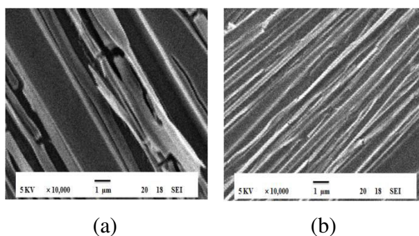
Figure II.34 : SnO 2 (al)/TX 1,5μl 300°C : a) 1h , b) 5h.
