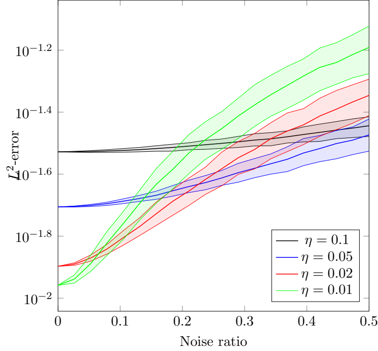
Figure 1.6: Error of the reconstructed permittivity in L^2(\Omega) with respect to the relative white noise on measurements. Each point is obtained by a statistic on 300 realizations of the noise. The lower and upper bounds of the colored parts represents the lower and upper decile.
