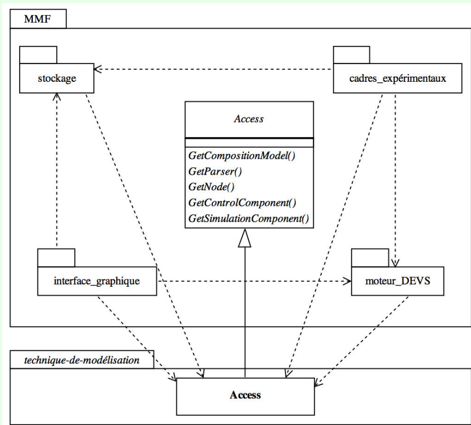
FIGURE 2.7 – Structure de JDEVS
