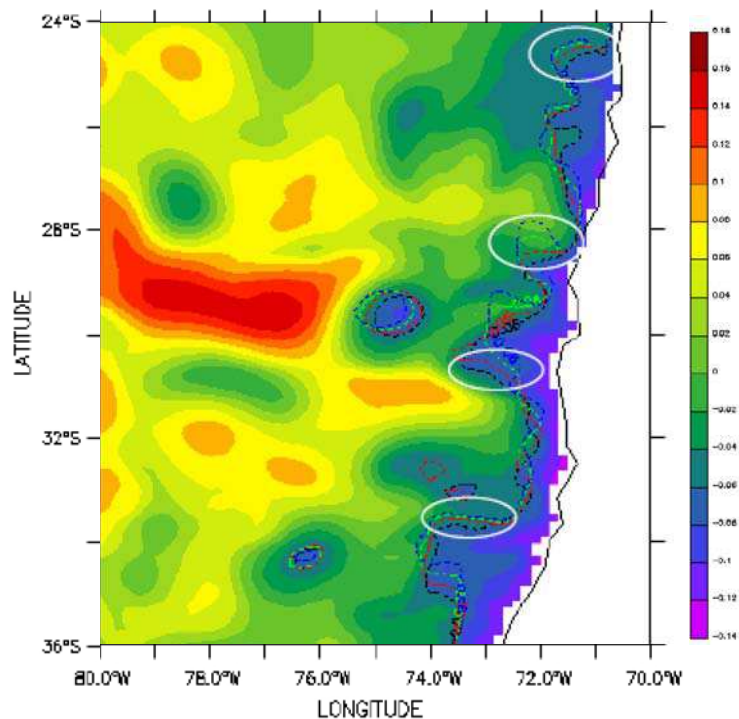
Fig. 1.5: Meanders of the upwelling front indicated on a map of SLA in the southern HCS simulated by the ROMS model (1/6° resolution, open boundary conditions from a global ocean model, atmospheric forcing from observed satellite winds and reanalyzed air/sea fluxes) for 19 th August 1995. Unit is meter. Contour interval is 0.02 m. The black, red, green and blue dashed lines indicate the position of the (-6 cm)-isoline on 19 th August, 24 th August, 29 th August, and 3 rd September 1995, respectively. White ellipses indicate the position of a few meanders ( V. Echevin, personal communication ).
