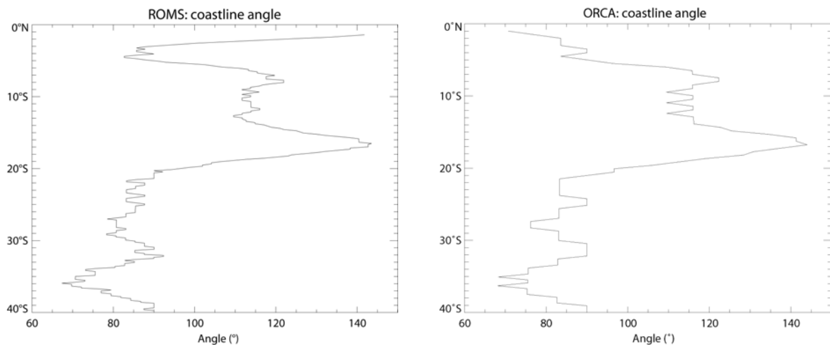
Fig. 3.14. Coastline angle relatively to the East direction between 1°S and 40°S for the ROMS (left) and ORCA (right) models.
