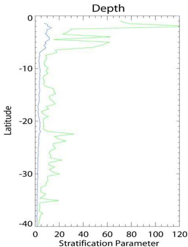
Fig. 3.25. Stratification parameter as a function of latitude ( ^{\circ} S) for ROMS (blue curve) and ORCA (green curve).
