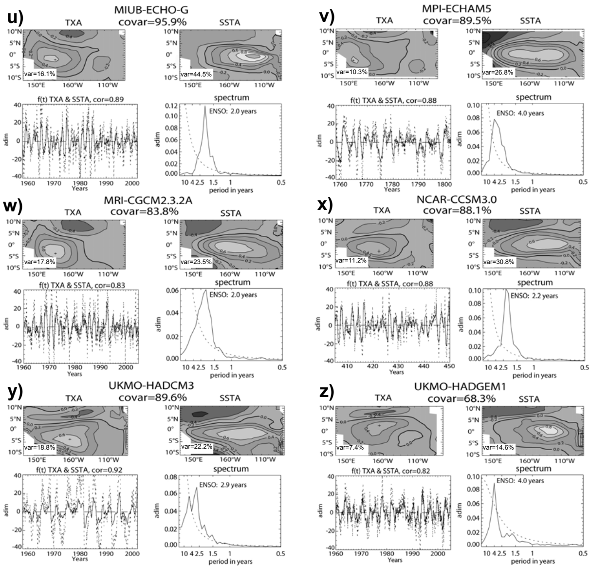
Fig. 1. First SVD mode between wind stress and SST anomalies (11°S-11°N, 134°E-81°W):
