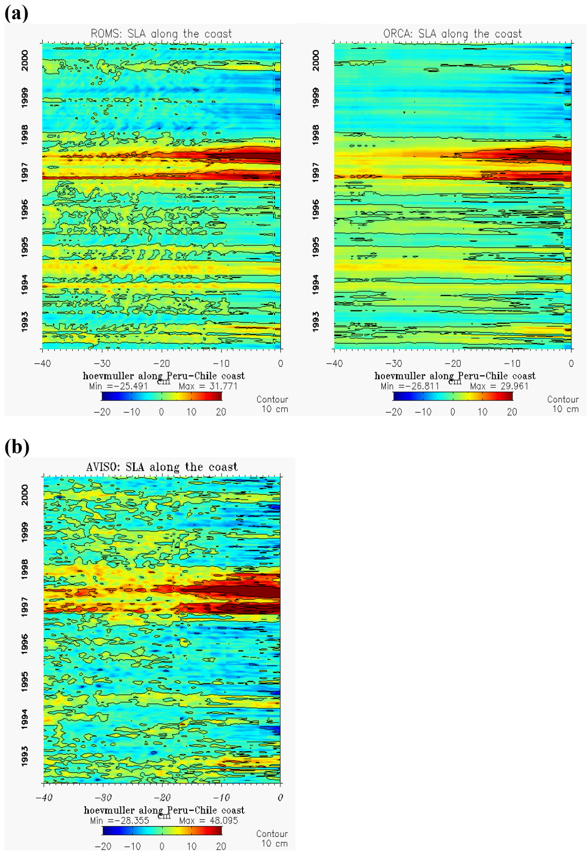
Fig. 3.10. SLA (cm) (a) simulated by ROMS (left panel), by ORCA (right panel) and (b) from AVISO altimetric data along the coast from 0°N to 40°S. Contour interval is 10cm.
