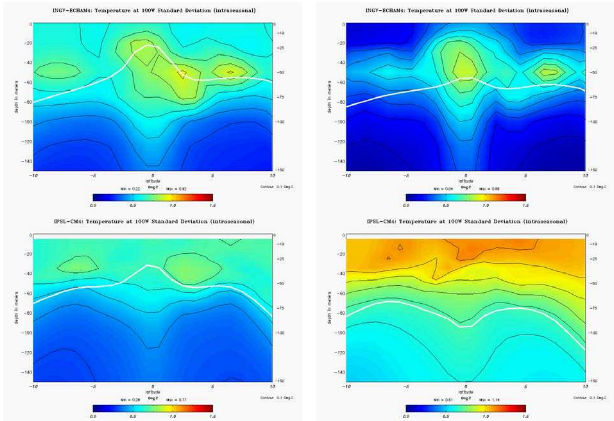
Fig. 4.4: same as fig. 4.3, but for intraseasonal temperature variability (RMS, ^\circ\text{C} ) at 100^\circ\text{W} ( 10^\circ\text{S} - 10^\circ\text{N} , 0m-150m). Contour interval is 0.1^\circ\text{C} . Colour scale is blue-red: 0– 1.5^\circ\text{C} .
