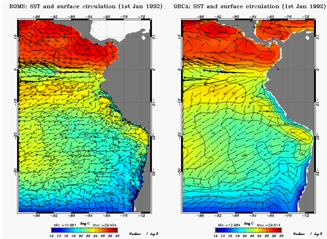
Fig. 3.5: SST ( ^{\circ}\text{C} ) and surface circulation (m/s) over the ESP for 1 st January 1992 as simulated by ROMS (left) and ORCA (right). Contour interval is 1^{\circ}\text{C} . The size (resp. direction) of the arrows (left and middle panels) is for the magnitude (resp. direction) of the surface currents.
