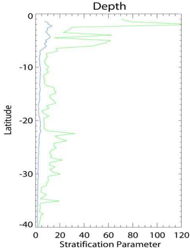
Fig. 3.25. Stratification parameter as a function of latitude (°S) for ROMS (blue curve) and ORCA (green curve).
