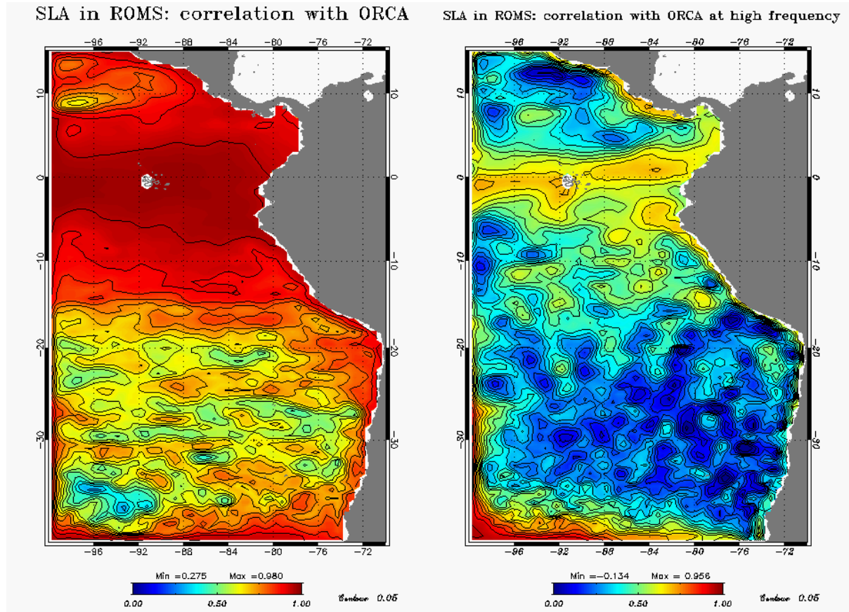
Fig. 3.11. Correlation maps between SLA simulated by ROMS and by ORCA. Left panel (resp. right panel) is for total (resp. high-pass filtered) SLA. Cut-off frequency is f_c = 150 days. Contour interval is 0.05.
