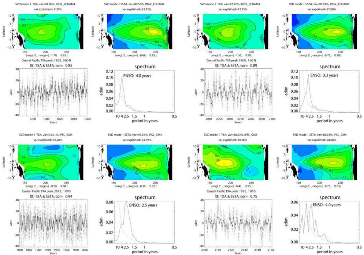
Fig. 4.8: First SVD mode between wind stress and SST anomalies (11°S-11°N, 134°E-81°W) for INGV-ECHAM4 (top) and IPSL-CM4 (bottom) under preindustrial (left) and 4xCO 2 climate (right). For each model simulation, from left to right and top to bottom: spatial patterns for zonal wind stress and SST anomalies, associated adimensionalized time series (full line for SST, dashed line for wind stress anomalies), and the corresponding frequency spectra adimensionalized by the energy integrated over the whole frequency domain (full line for SST anomalies, dashed line for red noise). CI = 0.2 units. Spatial patterns are adimensionalized by their respective variance over the domain and multiplied by 10. The location of maximum variance in wind stress anomalies is indicated by a cross on the map of the associated SVD mode. Percentage of explained variance for SST and zonal wind stress are indicated above the corresponding panels. Percentage of explained covariance is also provided. Correlation value between time series is indicated above the corresponding panel and the dominant ENSO period is mentioned on the spectrum plot.
