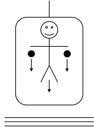
(c) The effect of a constant gravitational field: indistinguishable for our experimenter from that of a constant acceleration as in the previous figure.
