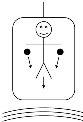
(e) The experimenter and his stones in a non-uniform gravitational field: the stones will approach each other slightly as they fall to the bottom of the elevator.
