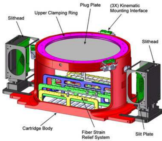
(a) BOSS cartridge schema
