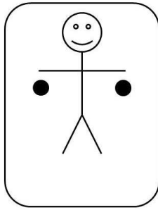
(a) An experimenter and his two stones freely floating somewhere in outer space, i.e. in the absence of forces.
