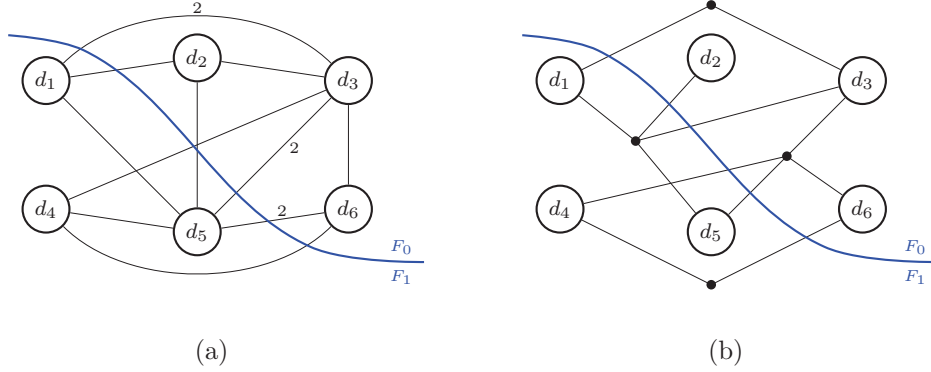
Figure 2.4: Graph models for data partitioning: (a) graph, (b) hypergraph
