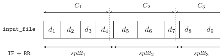
Figure 4.1: Input dataset and tuple assignments
