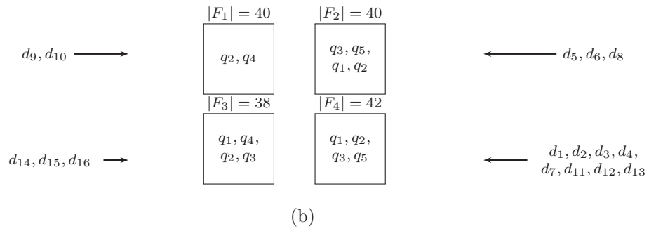
Figure 3.3: Example of execution of the distribution algorithms: a) algorithm DynPartGroup , b) algorithm DynPart
