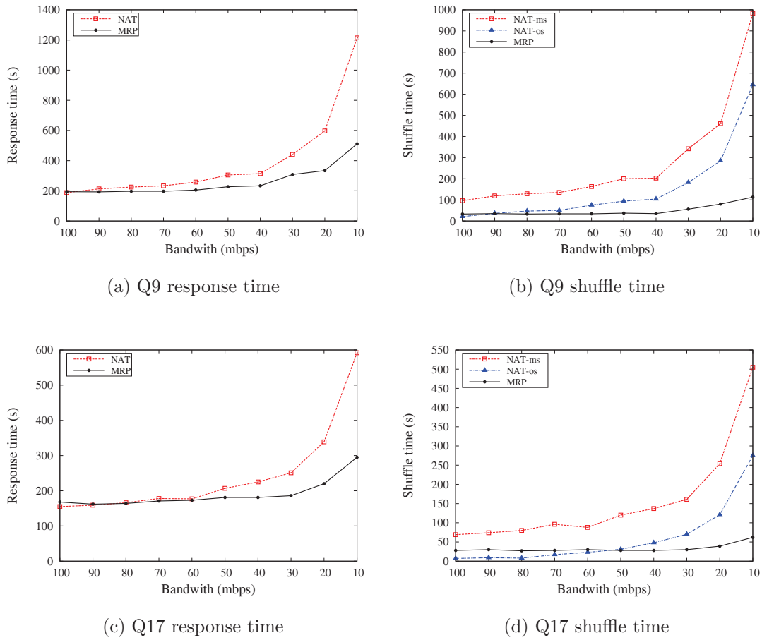
Figure 4.5: Results for varying network bandwidth in queries Q9 and Q17
