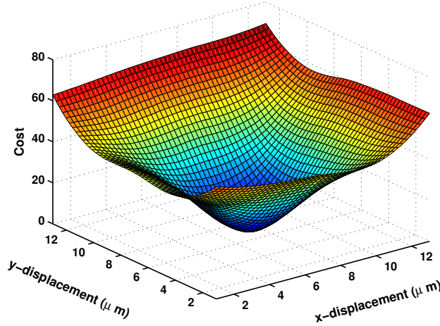
Figure 5.20: Cost function for Fourier-based visual servoing.
