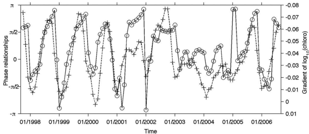
Figure 11. Temporal evolution of the mean meridional chlorophyll a gradient ( \log_{10}(\text{mgChl.m}^{-3}) \cdot \text{degree}^{-1} ) (dashed line with crosses, axis to the right) and the mean phase relationships between CHLA and SLA (solid line with circles, axis to the left) for latitudes located between 30^{\circ}\text{S} and 31^{\circ}\text{S} . The meridional chlorophyll a gradient is plotted with a reverse axis for ease of comparison.
