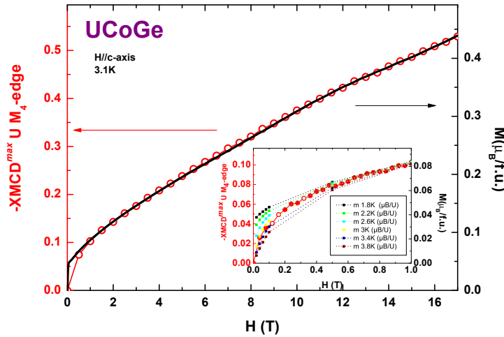
Figure 3.17 XMCD of the U M_4 -edge at 3K between 0T and 17T, \mathbf{H}/c , with the comparison with the macroscopic magnetization (right axis). In inset is shown the low field measurements, which enables to determine the temperature of the sample.
