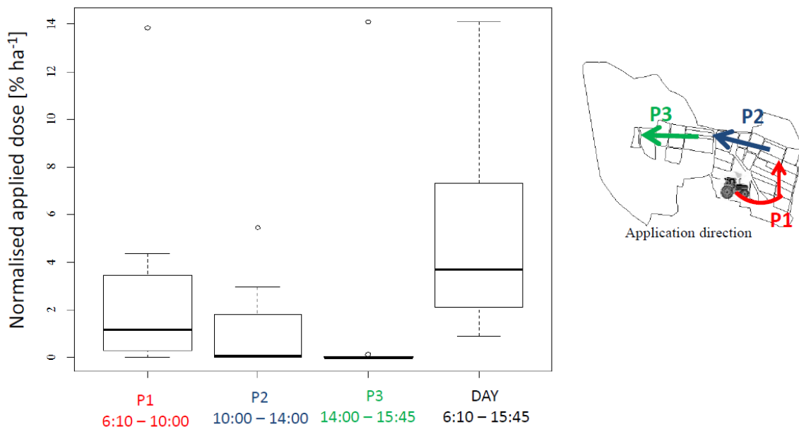
Figure III-4. Kresoxim methyl soil deposition of the nine collectors normalised by corresponding Thiessen area in the vineyard catchment (Rouffach, Alsace, France) during the three periods P1, P2 and P3 on May 24, 2011.
