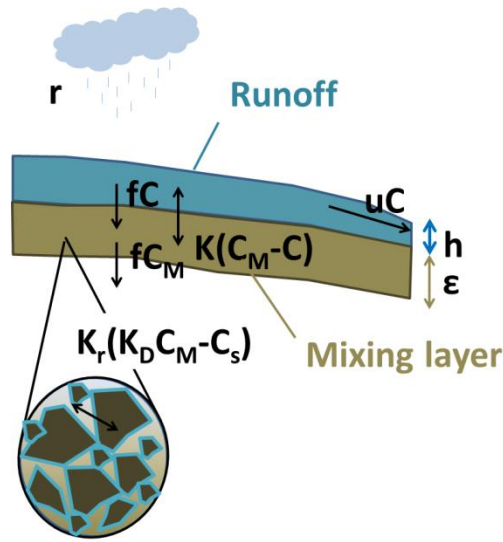
Figure V- 6. Conceptual mixing layer model for pesticide mobilisation (Adapted from Wallender (2008))
