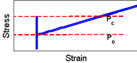
Figure IV.6 – Microscopic EOS for the hysteretic model. Transitions points are shown with dashed red lines and their values \vec{Z} = (P_o, P_c) are reported.
