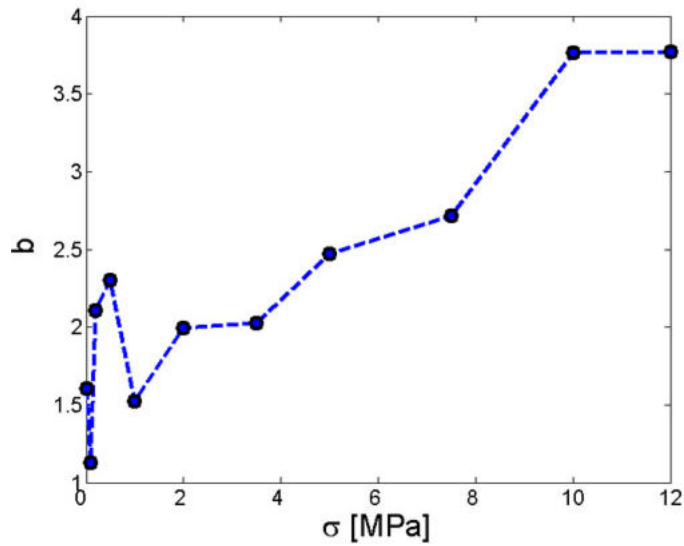
Figure IV.2 – Exponent b of the power law fitting function as a function of load. The increase of the exponent may be related to transitions to different damage conditions (progression of damage)[? ].
