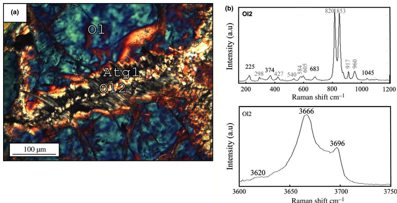
Fig. 5. (a) Microphotograph (cross polarized light) of an antigorite vein crossing an olivine with granoblastic secondary olivine (Ol2) at its centre. (b) Raman spectra of the granoblastic olivine. The secondary olivine possesses additional peaks (black values) corresponding to antigorite (usual peak values of olivine are in grey).
