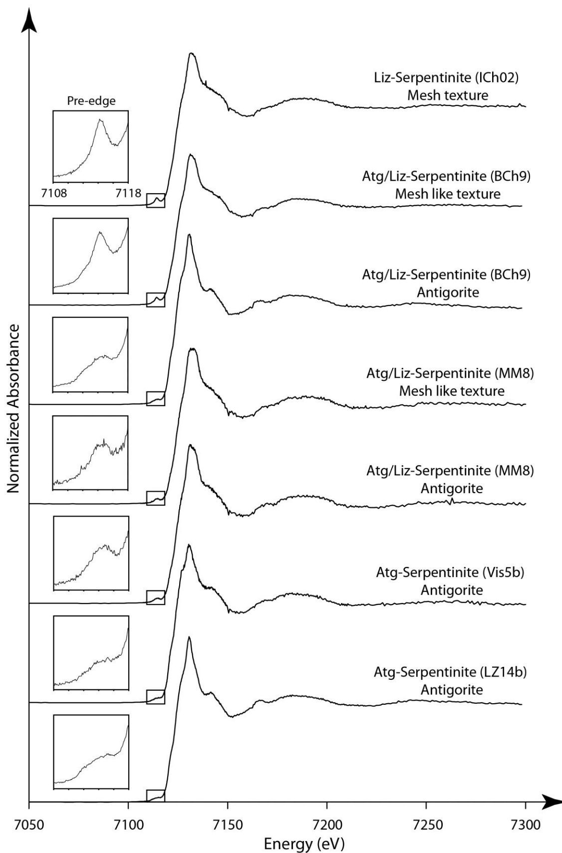
Figure 5: Spectral signature at the K-edge for the different serpentinite textures in the Montgenevre (ICh02, BCh9), Monte Maggiore (MM8), Monviso (Vis5b) and Lanzo (LZ14b) massifs. The box shows the pre-edge region of each XANES spectra.
