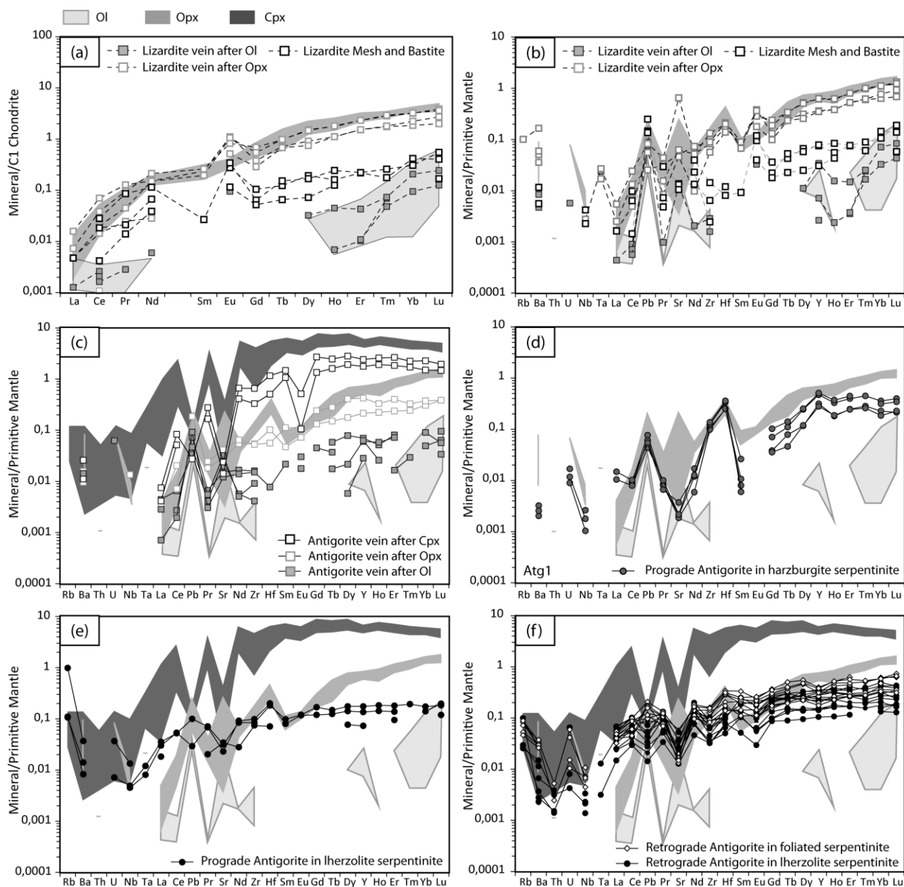
Fig. 6. Chondrite (a) and primitive mantle (b-c-d-e-f) normalized patterns for minerals composing the different lithologies of Lanzo massif. Normalising values are from Sun and McDonough (1989). Symbols are indicated in insert. (a) REE patterns of lizardite veins crossing the Opx and the OL and mesh and bastite texture from SSP. Host or destabilized mineral analyses are report in shaded area. (b) Spidergram of lizardite veins crossing the Opx and the OL and mesh and bastite texture from SSP. Host or destabilized mineral analyses are report in shaded area. (c) Spidergram of prograde antigorite veins crossing the Cpx, Opx and the OL from SSP. Host mineral analyses are report in shaded area. (d) Spidergram of prograde antigorite from massive serpentinite Group-1. Destabilized primary minerals are report in shaded area. (e) Spidergram of prograde antigorite from massive serpentinite Group-2. Destabilized primary minerals are report in shaded area. (f) Spidergram of retrograde antigorite from FS. Destabilized primary minerals are report in shaded area.
