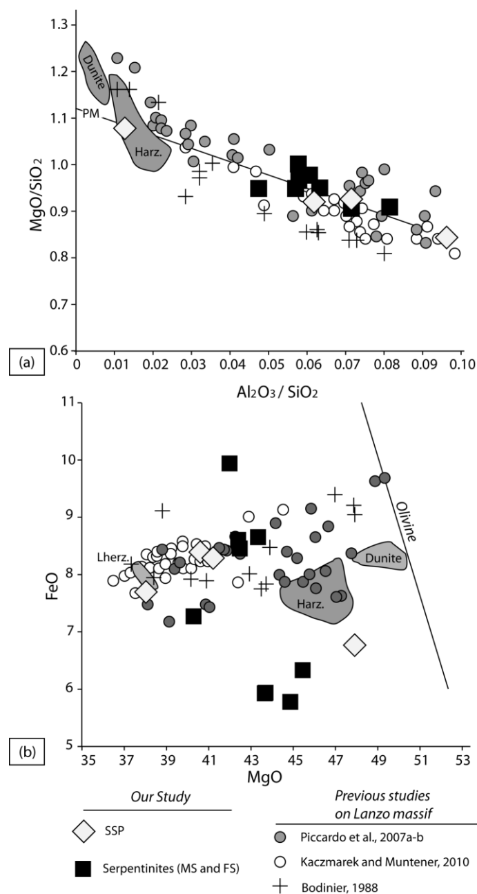
Fig. 4. Bulk rock major element composition of the SSP and serpentinites (MS and FS) illustrated in (a) Al_2O_3 versus MgO/SiO_2 and (b) MgO (wt%) versus FeO (wt%). On Fig. 4a, the dark line represents the silicate Earth differentiation trend and the primitive mantle ratio (PM, Kaczmarek and Muntener, 2010). On Fig. 4b, the dark line represents the stoichiometric variations of olivine Fe-Mg composition. Published data from Lanzo massif are shown for comparison: Bodinier (1988), Piccardo et al. (2007a, 2007b) and Kaczmarek and Muntener (2010). Abyssal peridotites poles (Lherzolite, Harzburgite and Dunites) are shown in shaded area and are from Godard et al. (2008).
