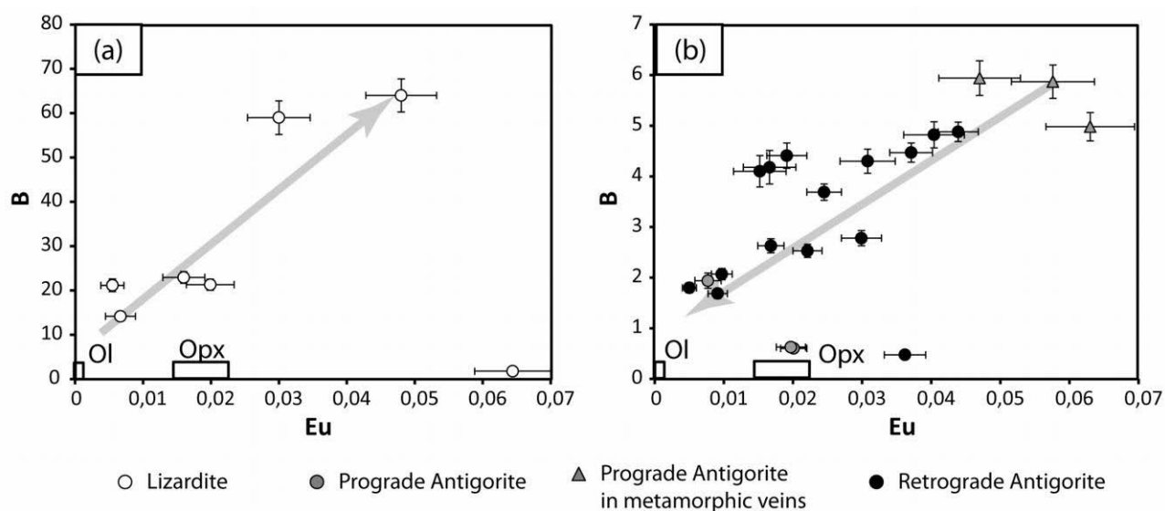
Fig. 10. (a) Plot of Eu versus B of lizardite of SSP. (b) Plot of Eu versus B of antigorite and secondary olivine composing the serpentinites (MS, FS and metamorphic veins) of Lanzo massif.
