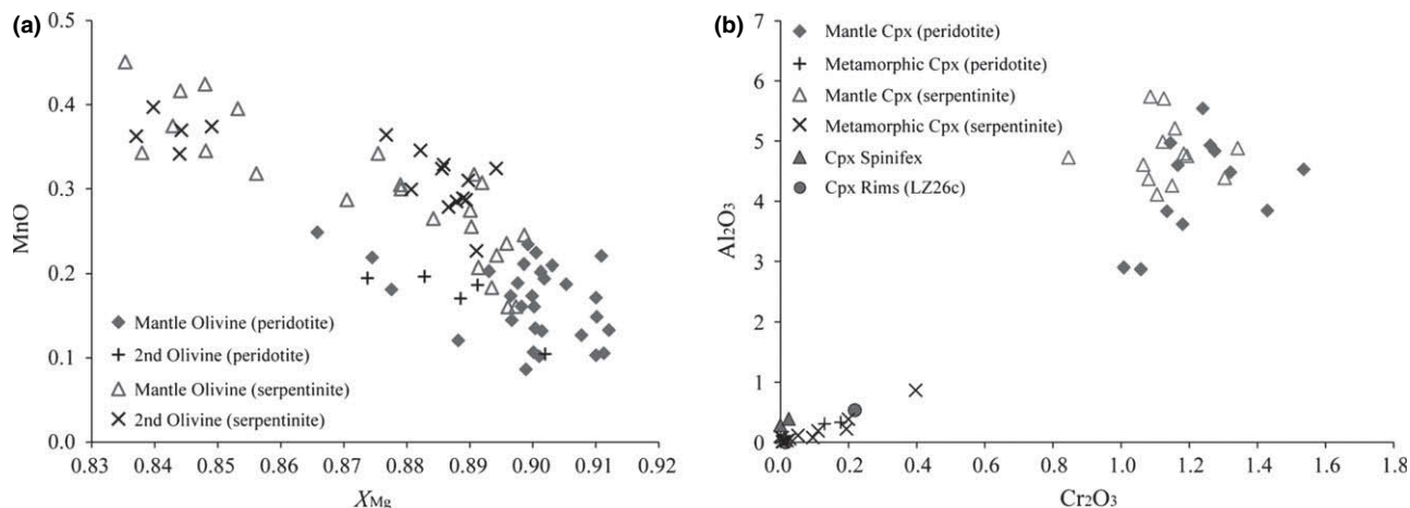
Fig. 4. (a) MnO (wt%) v. X_{Mg} contents of primary mantle olivine and secondary olivine (Ol 2 ) in slightly serpentinized peridotites and serpentinites. (b) Al_2O_3 (wt%) v. Cr_2O_3 (wt%) contents of primary clinopyroxene and metamorphic clinopyroxene in slightly serpentinized peridotites and serpentinites.
