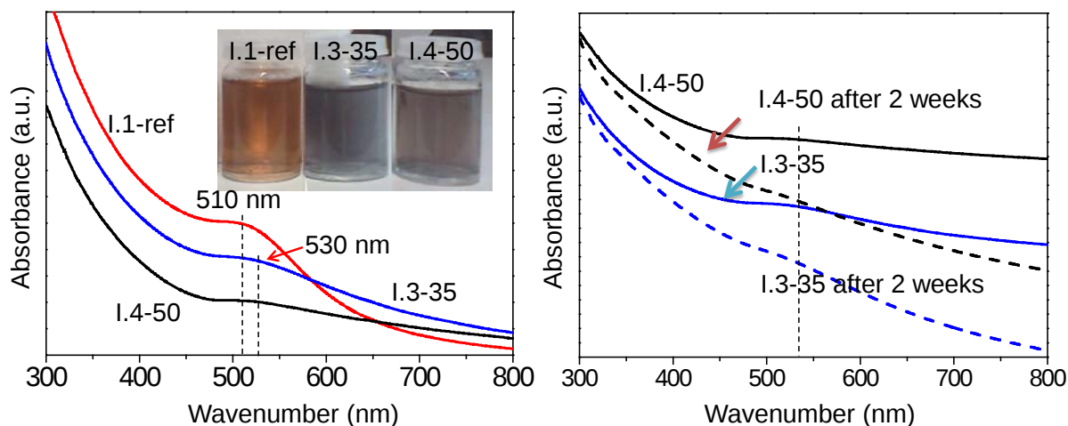
Figure 3.3 UV-vis spectra of Au colloids prepared at different temperature. [\text{NaBH}_4] = 0.1 \text{ M} , [\text{Au}] = 10^{-4} \text{ M} , \text{NaBH}_4 : Au = 5: 1 (molar ratio), PVA: Au= 5: 1 (weight ratio), reaction temperature for I.1-ref, I.3-35, and I.4-50 is 25°C, 35°C, and 50°C, respectively.
