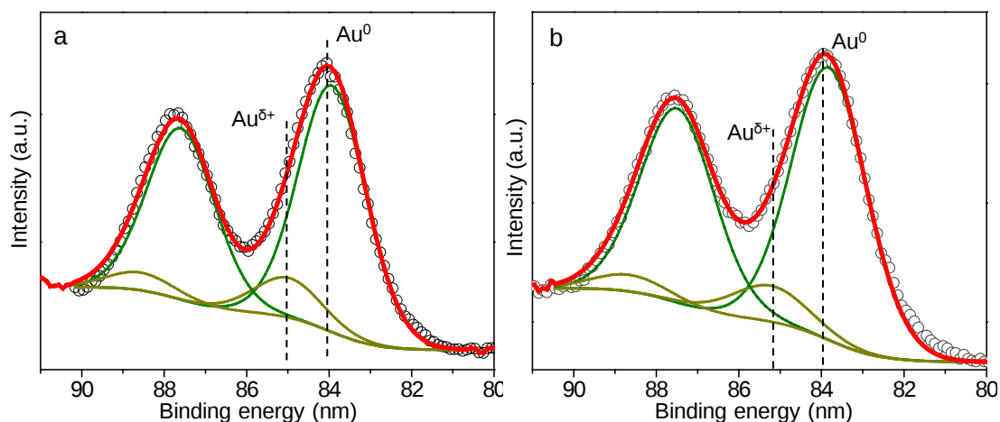
Figure 6.8 Au 4f XPS spectra of Au/SS5@Cu-C before (a) and after (b) selective oxidation of \text{H}_2\text{S} . The circle dots are the initial data, and the solid lines are the fitted lines.
