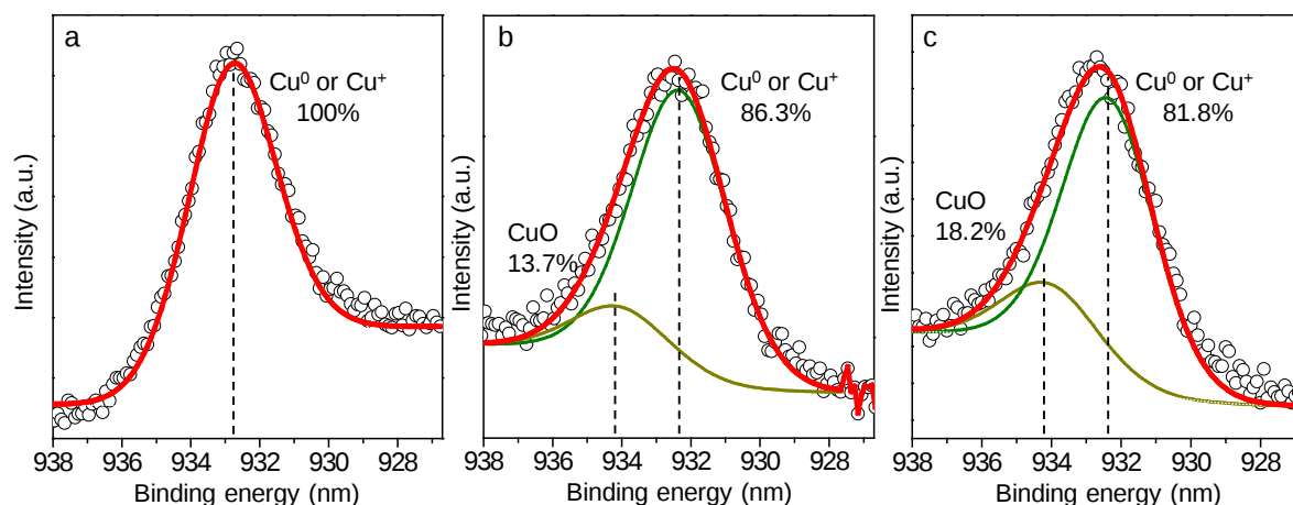
Figure 5.4 Typical deconvolution of Cu 2p_{3/2} XPS peak of fresh Au/SS5@Cu-C (a), Au/SS5@Cu-C after the first run of CO oxidation (b), and the spent Au/SS5@Cu-C after stability test (c). The balls illustrate the initial XPS spectrum, and the solid lines correspond to the fitted line.
