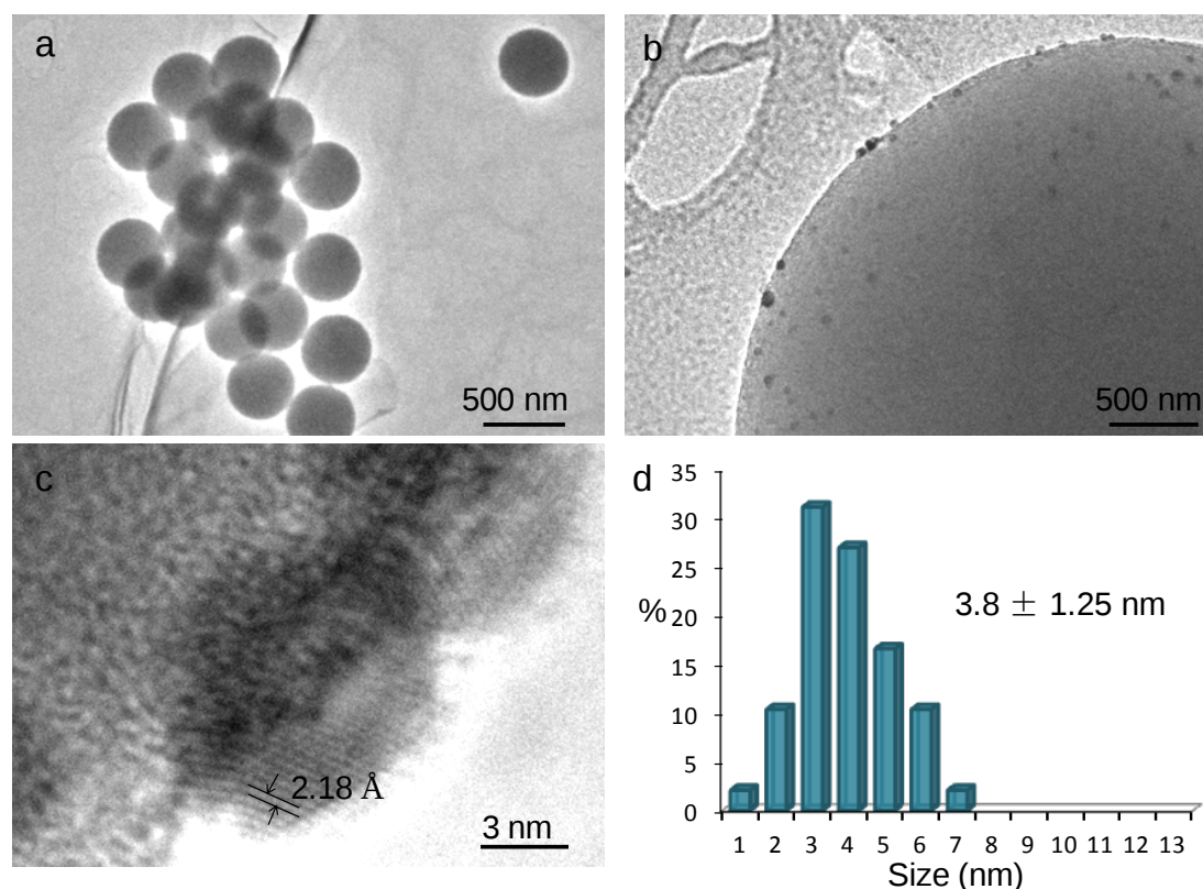
Figure 6.7 The TEM images and size distribution of spent \text{Au}/\text{SS5}@\text{Cu-C} sample.
