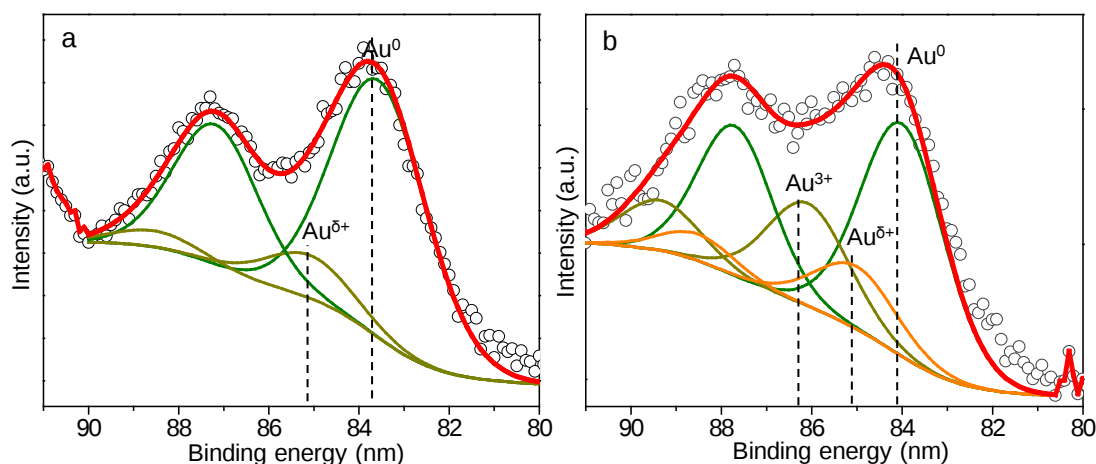
Figure 6.3 Au 4f XPS spectra of Au/SS5-C before (a) and after (b) selective oxidation of \text{H}_2\text{S} . The circle dots are the initial data, and the solid lines are the fitted lines.
