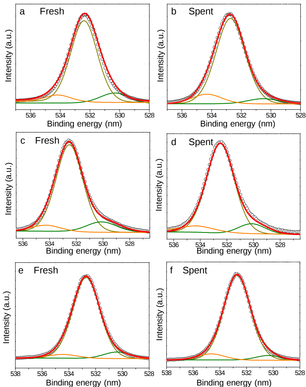
Figure 5.7 O 1s XPS spectra of fresh and spent Au/SS5@Cu-C (a-b), Au/SS5@Fe-C (c-d), and Au/SS5@Co-C (e-f) catalysts for CO oxidation. The balls illustrate the initial XPS spectrum, and the solid lines correspond to the fitted line.
