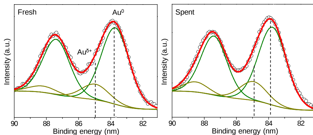
Figure 5.6 XPS profiles of Au 4f over fresh and spent Au/SS5@Co-C catalysts after three times of CO oxidation from T_{\text{room}} to 300°C. The balls illustrate the initial XPS spectrum, and the solid lines correspond to the fitted line.
