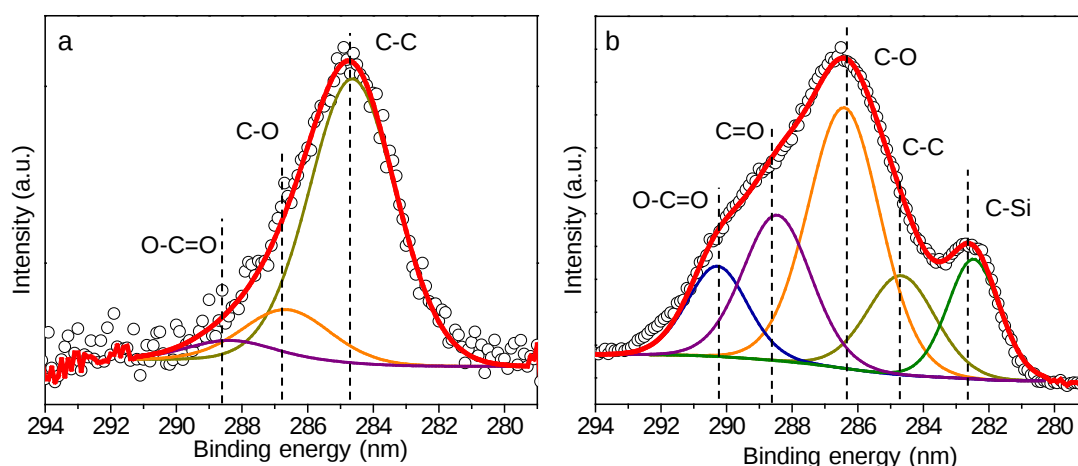
Figure 6.5 The C 1s XPS spectra of Au/SS5-C before (a) and after (b) selective oxidation of \text{H}_2\text{S} . The circle dots are the initial data, and the solid lines are the fitted lines.
