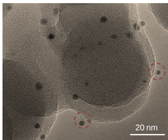
Figure 4.7 TEM image of Au/SS1. In this sample, Au-NPs about 3 nm was successfully loaded on the surface of SS1 support without addition of any organic couplant. The nanoparticles in the red circle on the surface of support are captured by the glue-like stuff, which is inferred to be the PVA.
