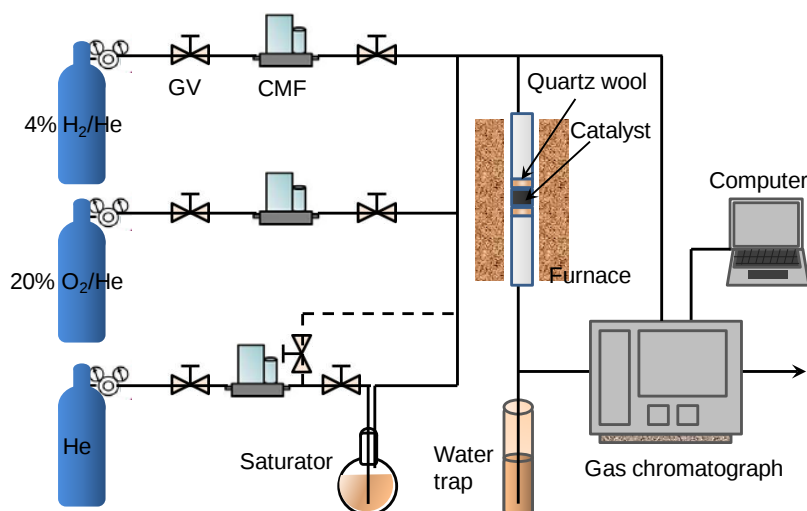
Figure 2.7 Schematic diagram of the apparatus for selective \text{H}_2\text{S} oxidation.
