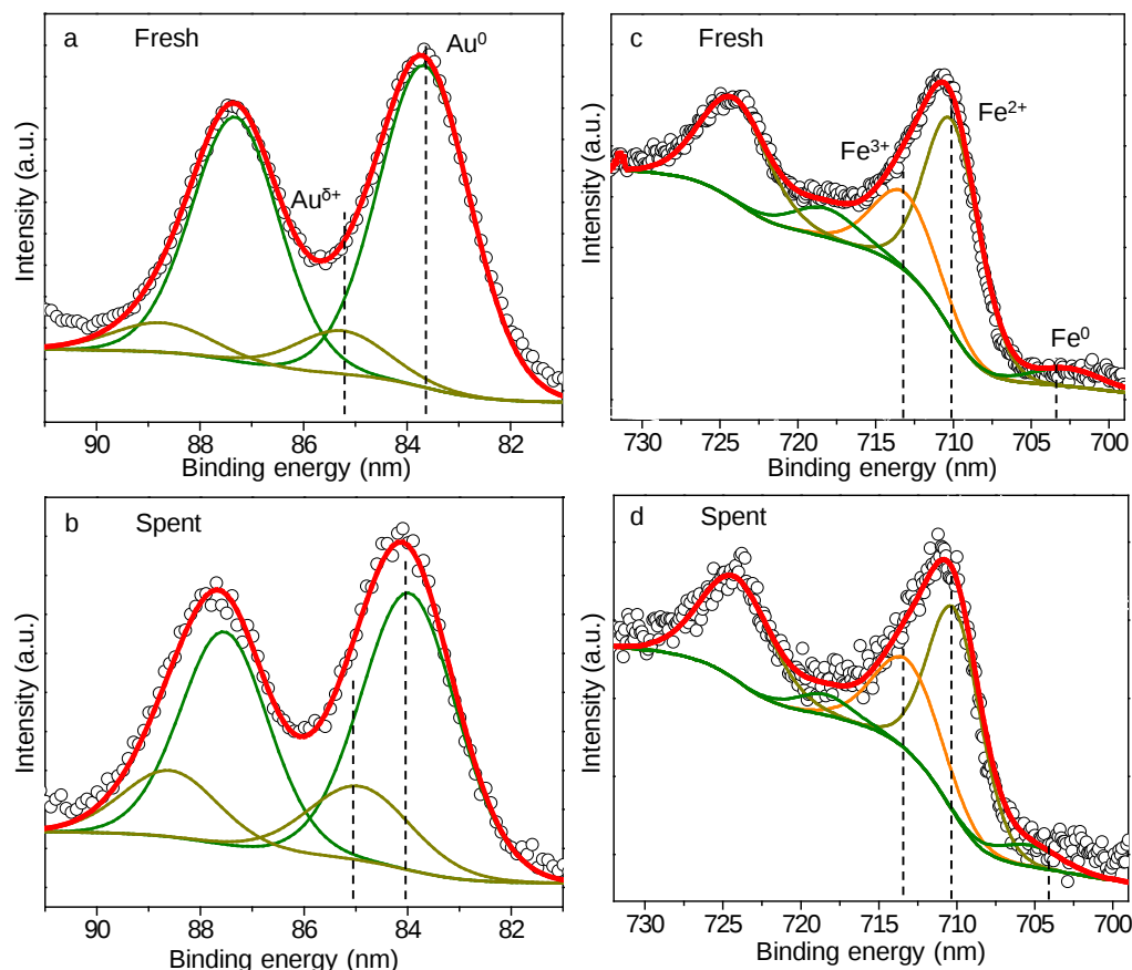
Figure 5.5 XPS profiles of Au4f (a-b) and Fe 2p (c-d) over fresh and spent Au/SS5@Fe-C catalysts after three times of CO oxidation from T_{room} to 300°C. The balls illustrate the initial XPS spectrum, and the solid lines correspond to the fitted line.
