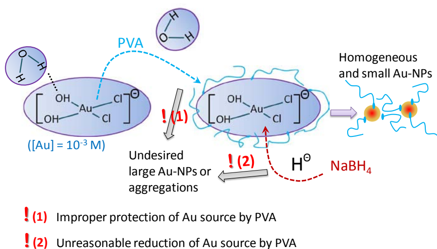
Schema 3.1 The possible paths for Au-NPs formation during synthesize of gold colloid in water at room temperature.
