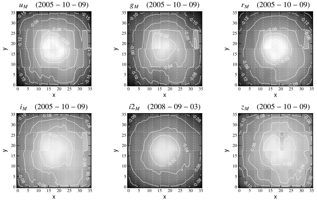
Figure 2.10: Map of the photometric corrections relative to the twilight flat fields using dithered observations of dense stellar fields. Each panel represents the \delta zp(\mathbf{x}) map for the entire focal plane (CCD#0 up left, #35 down right). The corrections are large, typically 10% from center to corner (figure taken from Betoule et al., 2012 )
