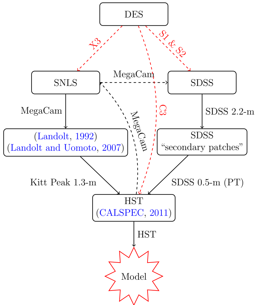
Figure 2.13: Redundant calibration chains explored by the SNLS and SDSS-II surveys. The black arrows draw the paths initially set by (Regnault et al., 2009) (SNLS) and (Holtzman et al., 2008) (SDSS-II). The red dashed arrows shows the paths opened by Betoule et al. (2012).
