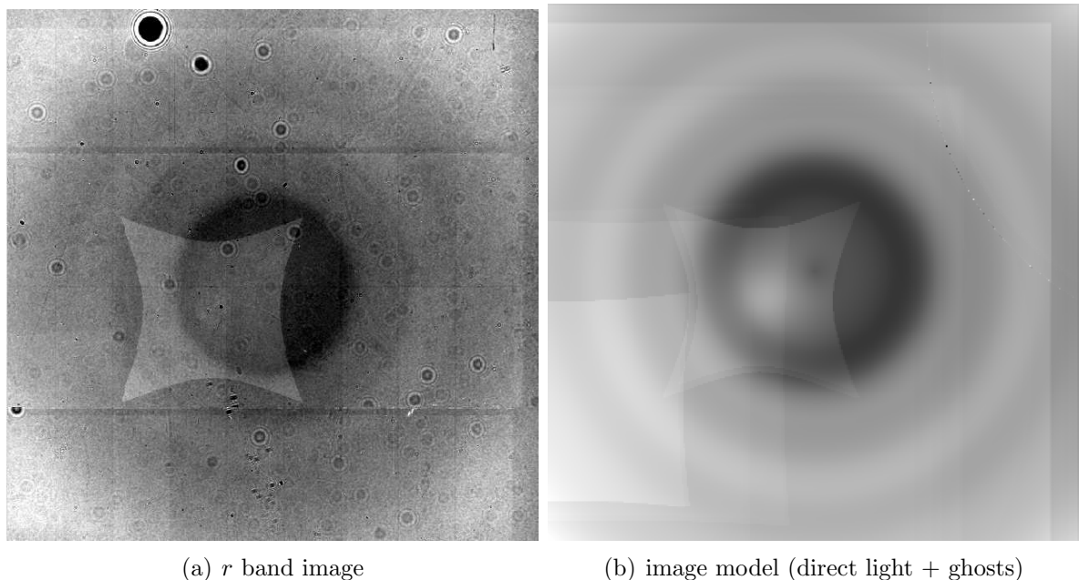
Figure 3.12: Left: MegaCam/SnDICE calibration frame, taken in the r band, with a LED that covers the filter front. The ghosts are clearly apparent. In particular, we clearly see the reflection of the focal plane CCDs on the filter and the cryostat window. Right: model of the same exposure, computed with the MegaCam optical simulation. The reflectivity of some lenses has been slightly increased, so that the fainter ghosts can be clearly seen.
