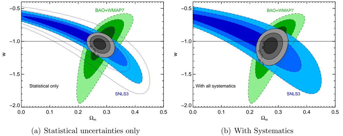
Figure 1.7: Confidence contours in the \Omega_m - w plane, assuming a flat Universe and a constant w . The SNLS constraints are shown in blue. The BAO + WMAP7 constraints (Komatsu et al., 2011; Percival et al., 2010) are represented in green. The systematics represent slightly more than half of the total error budget. They are essentially due to photometric calibration.
