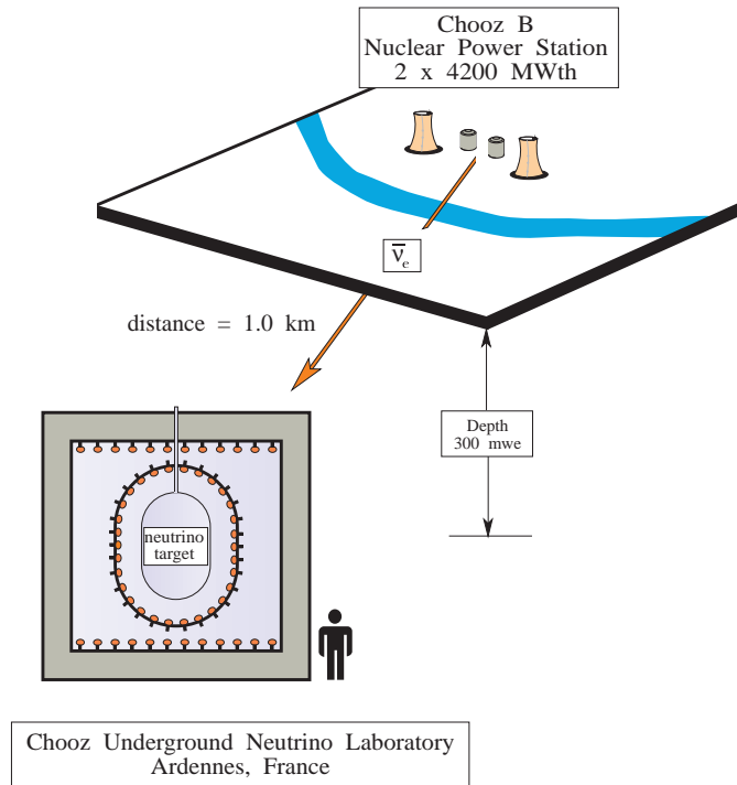
Figure 3.17: Chooz experimental site overview [94, 95].
