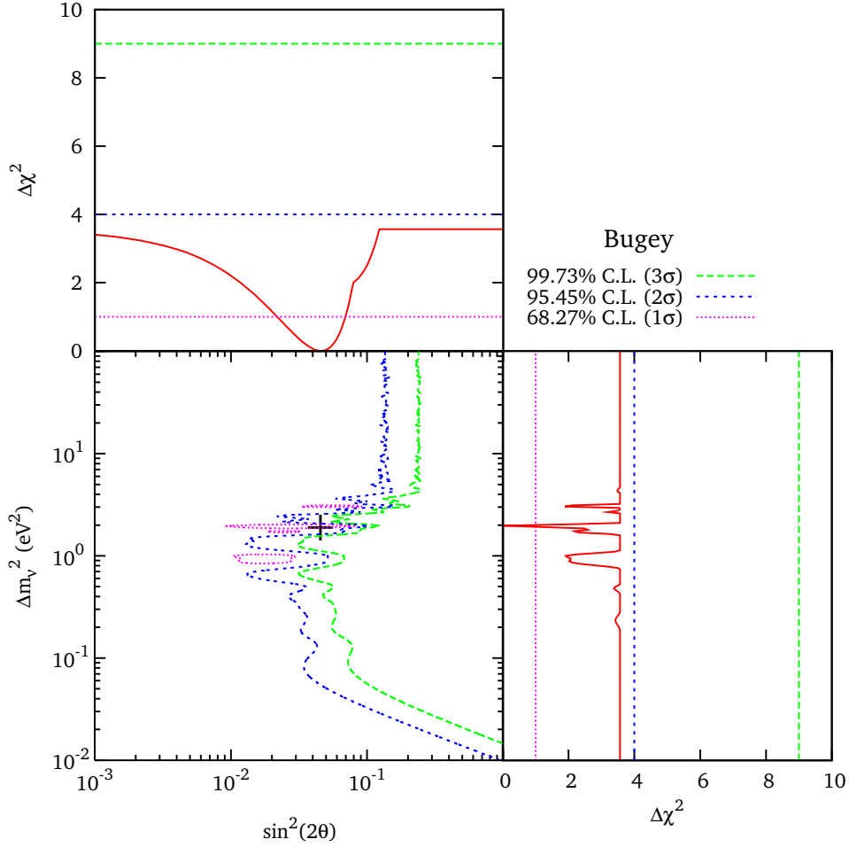
Figure 3.14: Allowed regions in the oscillation parameter space and marginal \Delta\chi^2 's for \sin^2 2\theta and \Delta m^2 obtained from the least-squares analysis of the Bugey data. The best fit point corresponding to \chi_{\min}^2 is indicated by a cross.
