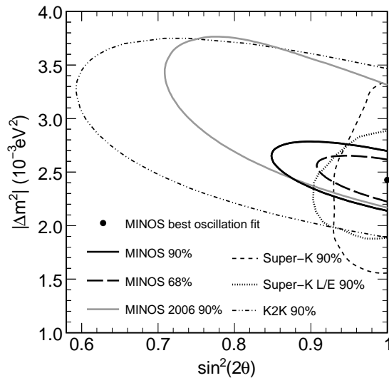
Figure 2.4: Allowed region of the oscillation parameters using the MINOS results, and compared to other experiment results [61].
