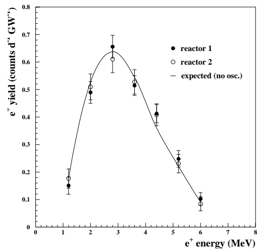
Figure 3.20: Positron yields for the two reactors, as compared with the expected yield for no oscillations [96].
