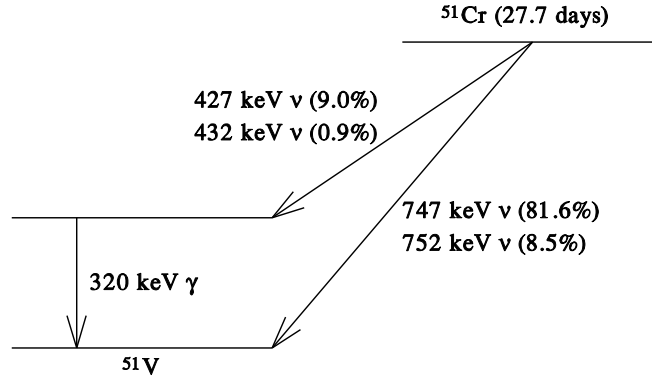
Figure 3.1: Decay scheme of the ^{51}\text{Cr} radioactive source [82].
