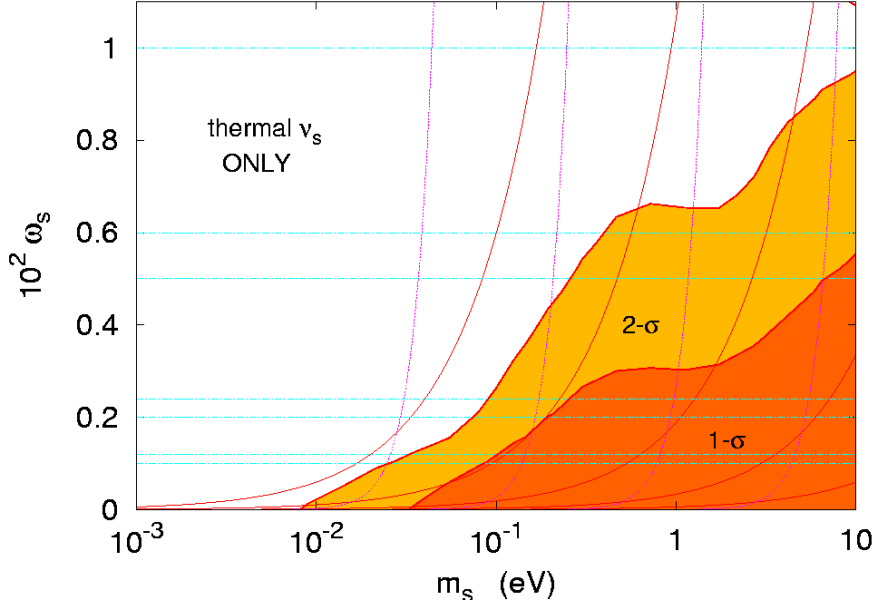
Figure 5.13: Same to figure 5.12 with, in addition, the regions allowed at the 68.3% ( 1\sigma ) and 95.4% ( 2\sigma ) C.L. by our cosmological data set, in a Bayesian analysis with flat priors on \log_{10}(m_s) and \omega_s within the displayed range.
