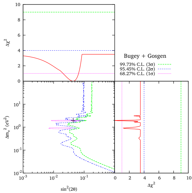
Figure 4.10: Allowed regions in the oscillation parameter space and marginal \Delta\chi^2 s for \sin^2 2\theta and \Delta m^2 obtained from the combined fit of the Bugey and Gosgen nuclear reactor experiments. The best fit point corresponding to \chi_{\min}^2 is indicated by a cross.
