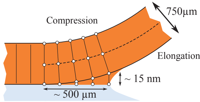
Fig. 5: Schematic representation of the wafer profile near the bonding front. The solid line gives the shape predicted by the thin plate theory. The colored area is the expected real shape. Vertical line represents the normal to the neutral axes line. The upper wafer surface is compressed, while the inner surface is elongated, with respect to the neutral axis. Because the vertical displacement due to the adhesion forces is small in comparison to the plate deformation, the horizontal elongation is expected to remain when both surfaces are pulled into contact. It should be noted, that the scale of this picture is exaggerated. The expected wafer thickness variation is more than one thousand time smaller than the wafer thickness. The real order of magnitude associated to this problem is addressed at the end of the section.
