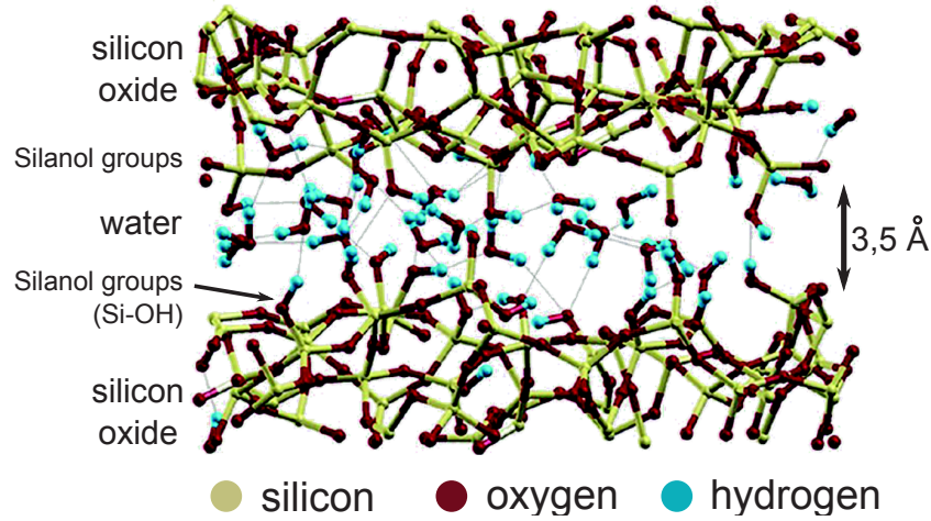
Fig. 5: Schematic representation of the bonding interface obtained from a molecular dynamic simulation (from S. Leroy et al. [39]). Grey lines account for hydrogen bonds.
