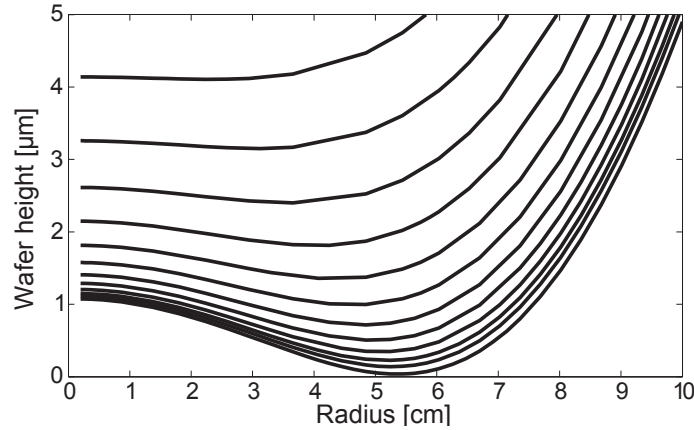
Fig. 19: Final time step of “before initiation” step for a positive initial curvature (here bow = +37.5 \mu m ). The spontaneous contact is no longer located at the wafer center, but is a concentric ring. An air bubble is then expected to be trapped in the central region of the wafer.
