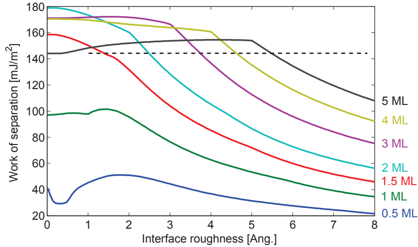
Fig. 6: Variation of the theoretical work of separation values calculated from the molecular dynamics results as a function of the interface roughness for different amount of water at the interface (these values are twice those given by D. J. Cole et al. because, here, the interface is considered). The dashed line indicates twice the surface tension of water.
