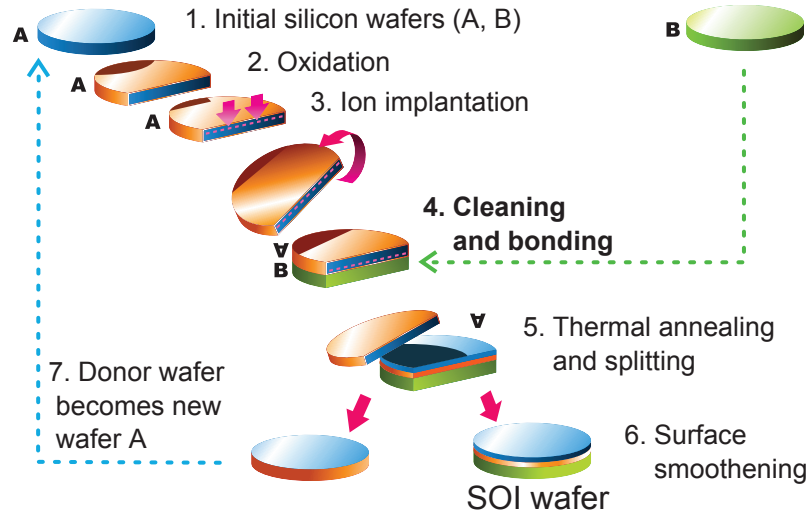
Fig. 1: Schematic representation of the Smart-Cut™ process. The silicon-on-insulator wafer is a silicon wafer having on its surface a thin ( < \sim 1 \mu m ) single crystalline silicon layer lying over a insulating layer (amorphous silicon oxide).
