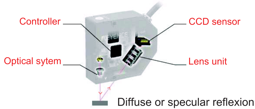
Fig. 9: Measurement principle using triangulation (from the Keyence catalog). The size of the sensor is about 6 \times 6 \times 3\ cm and the distance from the substrate to the sensor is about 2\ cm .
