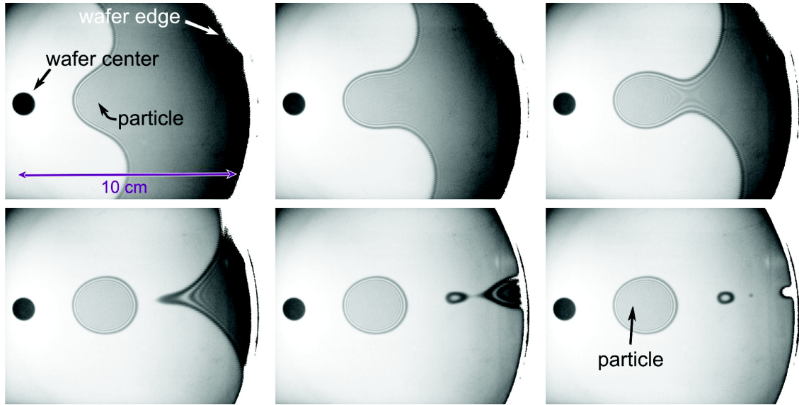
Fig. 11: Observations of the bonding front propagation when a punctual particle is present on the wafer surface. Delay between images is 1 \text{ s} . The final bubble is neither centered around the particle, nor circular.
