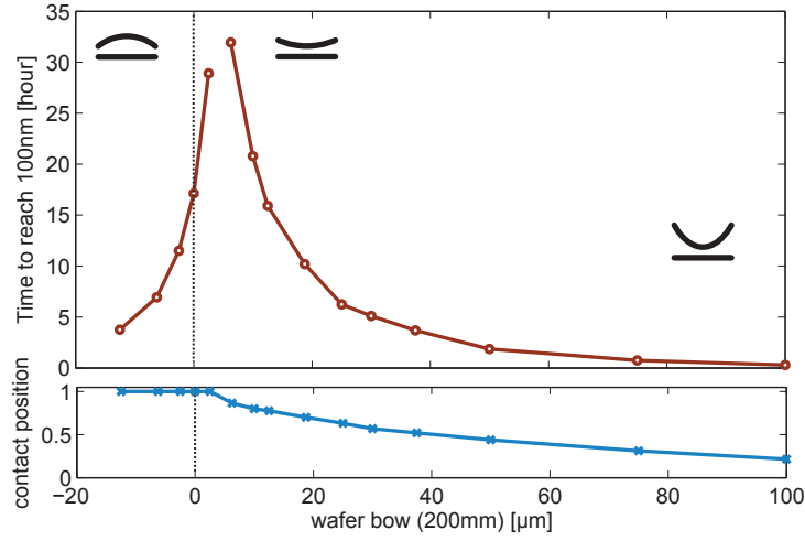
Fig. 18: Variation of the time needed to reach a gap of 100 nm as a function of the initial bow (both concave and convex shape). The contact position is the radius where the contact should occurs, normalized by the wafer radius. Computation is performed for 200 mm diameter wafer.
