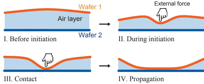
Fig. 5: Sequence of direct wafer bonding I. before initiation only gravity and fluid pressure act on the top wafer; II. an external initiation force is locally applied; III. contact occurs between the wafers at the point of initiation while holding the applied force; IV. adhesion forces lead to the expansion of the bonded area.
