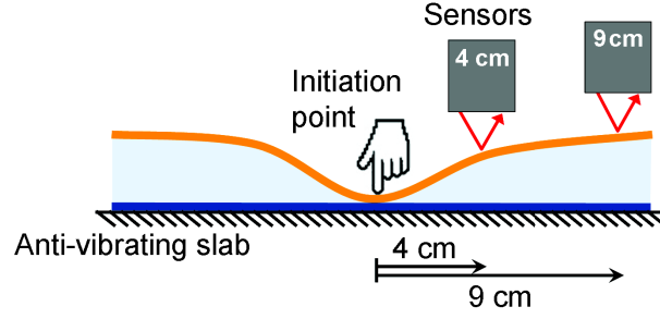
Fig. 10: Schematic of the experimental setup to measure out-of-plane bonding wafer displacement.
