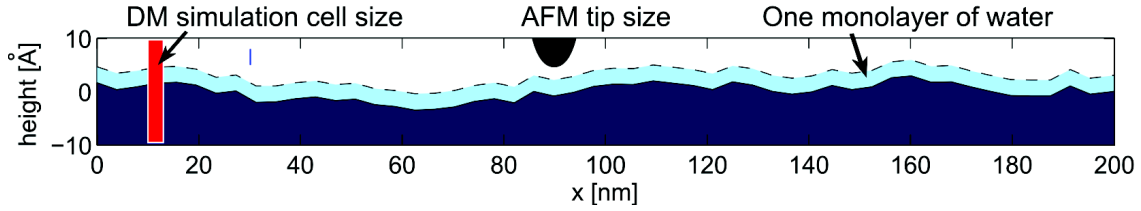
Fig. 1: The dark area is a small part of an experimental AFM profile. Each point is located at every \Delta x \approx 40 \text{ \AA} ( 2 \mu m long scan for 512 points). The dashed line represents one monolayer of water molecules ( 3 \text{ \AA} ) and the rectangle represents the box size of the molecular dynamic simulation ( 30 \times 30 \times 20 \text{ \AA}^3 ). The AFM tip radius is typically about 10 nm . It should be noted that the x-axis scale is ten times larger than the z-axis scale. The roughness value for the entire AFM scan ( 2 \times 2 \mu m^2 ) is about 1 \text{ \AA RMS} .
