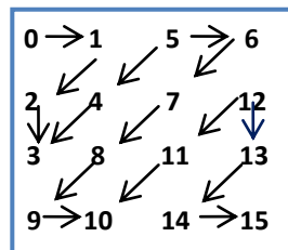
Figure A-8: Zig-zag scanning.
