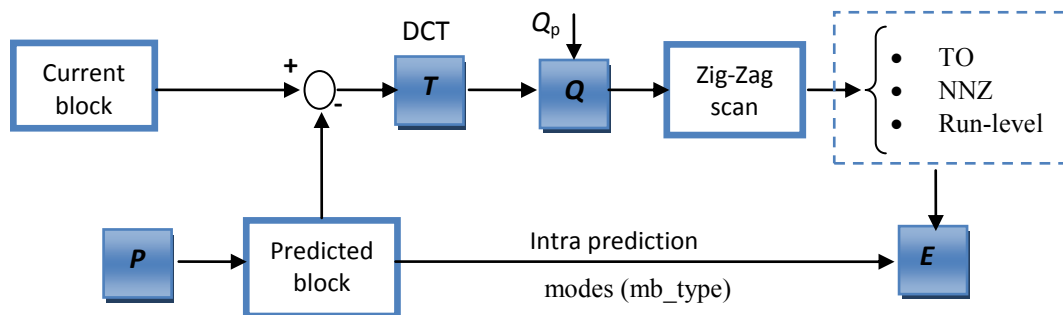
Figure II-37: Intra frame coding diagram.
