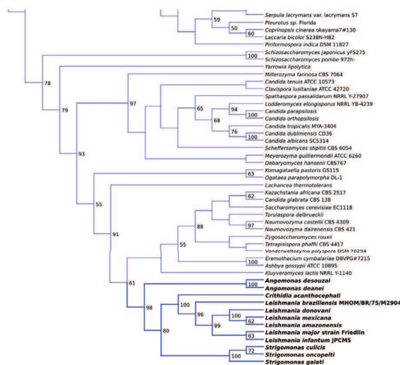
Figure C.20: Maximum likelihood phylogeny of arginase (EC:3.5.3.1). Overall tree colored according to taxonomic affiliation of sequences. Values on nodes represent bootstrap support (only 50 or greater shown) and distance bar only applies to the overall tree and not to the detailed regions.
