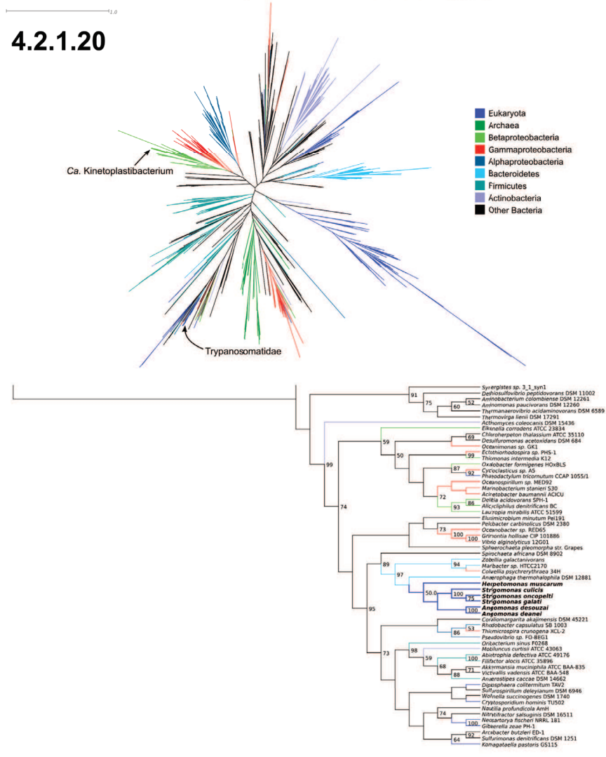
Figure C.15: Maximum likelihood phylogeny of (EC:4.2.1.20). Overall tree colored according to taxonomic affiliation of sequences. Values on nodes represent bootstrap support (only 50 or greater shown) and distance bar only applies to the overall tree and not to the detailed regions.
