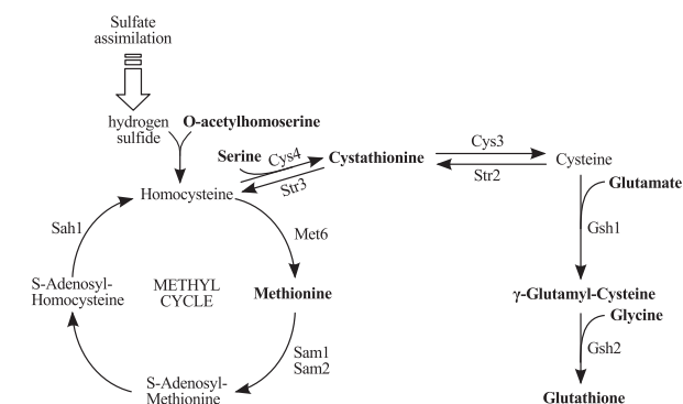
Fig. 1. Glutathione biosynthetic pathway. Compounds in bold are discriminating in Madalinski et al. (2008) and are involved in the synthesis of glutathione. Source: adapted from Figure 1 in Lafaye et al. (2005)
