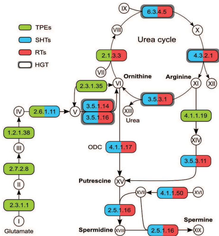
Figure 2.7: Arginine, ornithine, and polyamine synthesis pathway. Enzymes surrounded by a thick gray box were shown to be horizontally transferred from Bacteria (see main text). Metabolites – I: glutamate; II: N-acetylglutamate; III: N-acetylglutamyl-phosphate; IV: N-acetyl-glutamate semialdehyde; V: N-acetylornithine; VI: ornithine; VII: carbamoyl-phosphate; VIII: citrulline; IX: aspartate; X: arginino succinate; XI: arginine; XII: fumarate; XIII: urea; XIV: agmatine; XV: putrescine; XVI: S-adenosylmethionine; XVII: S-adenosylmethioninamine; XVIII: spermidine; XIX: spermine. Enzymes – 2.1.3.3: ornithine carbamoyltransferase; 6.3.4.5: argininosuccinate synthase; 4.3.2.1: argininosuccinate lyase; 3.5.3.1: arginase; 4.1.1.17: ornithine decarboxylase; 3.5.1.14: aminoacylase; 3.5.1.16: acetylornithine deacetylase; 2.3.1.35: glutamate N-acetyltransferase; 2.6.1.11: acetylornithine aminotransferase; 1.2.1.38: N-acetyl-gamma-glutamyl-phosphate reductase; 2.7.2.8: acetylglutamate kinase; 2.3.1.1: amino-acid N-acetyltransferase; 3.5.3.11: agmatinase; 4.1.1.19: arginine decarboxylase; 4.1.1.50: adenosylmethionine decarboxylase; 2.5.1.16: spermidine synthase.
