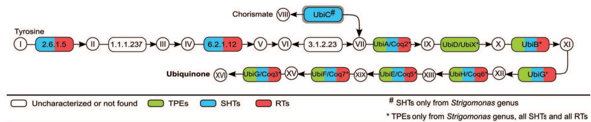
Figure 2.20: Ubiquinone biosynthesis Enzymes surrounded by a gray box were possibly acquired through horizontal transfer from Bacteria to trypanosomatids (see main text). Metabolites - I : L-Tyrosine; II : 4-Hydroxyphenylpyruvate; III : 4-Hydroxyphenyllactate; IV : 4-Coumarate; V : 4-Coumaroyl-CoA; VI : 4-Hydroxybenzoyl-CoA; VII : 4-Hydroxybenzoate; VIII : Chorismate; IX : 4-Hydroxy-3-polyprenylbenzoate; X : 2-Polyprenylphenol; XI : 2-Polyprenyl-6-hydroxyphenol; XII : 2-Polyprenyl-6-methoxyphenol; XIII : 2-Polyprenyl-6-methoxy-1,4-benzoquinone; XIV : 2-Polyprenyl-3-methyl-6-methoxy-1,4-benzoquinone; XV : 2-Polyprenyl-3-methyl-5-hydroxy-6-methoxy-1,4-benzoquinone; XVI : Ubiquinone. Enzymes - 2.6.1.5: tyrosine aminotransferase; 1.1.1.237: hydroxyphenylpyruvate reductase; 6.2.1.12: 4-coumarate-CoA ligase; 3.1.2.23: 4-hydroxybenzoyl-CoA thioesterase; UbiC: chorismate lyase; UbiA/Coq2: 4-hydroxybenzoate polyprenyltransferase; UbiD/UbiX: 3-octaprenyl-4-hydroxybenzoate carboxy-lyase; UbiB: ubiquinone biosynthesis protein; UbiG (EC:2.1.1.222): 2-polyprenyl-6-hydroxyphenyl methylase; UbiH/Coq6: 2-octaprenyl-6-methoxyphenol hydroxylase ; UbiE/Coq5: ubiquinone biosynthesis methyltransferase; UbiF/Coq7: 2-octaprenyl-3-methyl-6-methoxy-1,4-benzoquinol hydroxylase; UbiG/Coq3 (EC:2.1.1.64 / EC:2.1.1.114): 3-demethylubiquinol 3-O-methyltransferase / hexaprenyldihydroxybenzoate methyltransferase.
