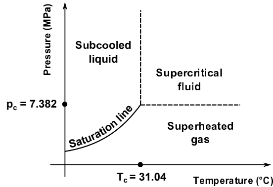
Figure 5.47: Phase diagram of carbon dioxide (CO 2 ). Dashed lines are only drawn to identify regions with different customary naming conventions. They do not signify phase transitions, as all fluid properties vary smoothly and continuously across these lines, (Pruess, [2006]).
