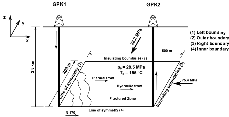
Figure 5.4: Geometric layout of the fractured zone to be stimulated at the HDR reservoir of Soultz–Sous–Forêts. GPK2 is drilled in the direction of fracture evolution. Only quarter of the problem is to be studied due to symmetry.
