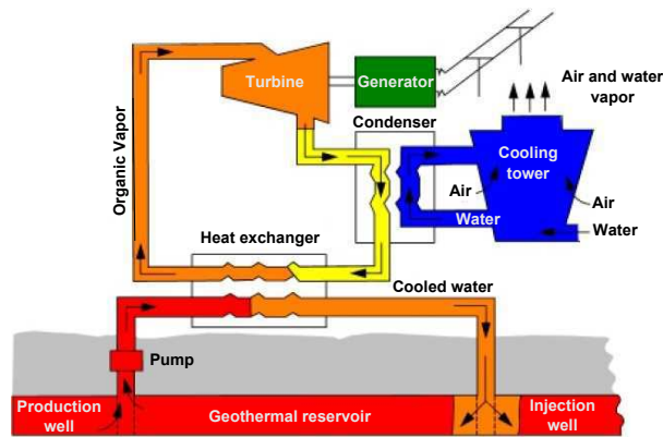
Figure 1.11: Binary power or organic Rankine cycle plant using a low temperature geothermal resource and a secondary fluid of a low boiling-point hydrocarbon edited from (Lund, [2007]).
