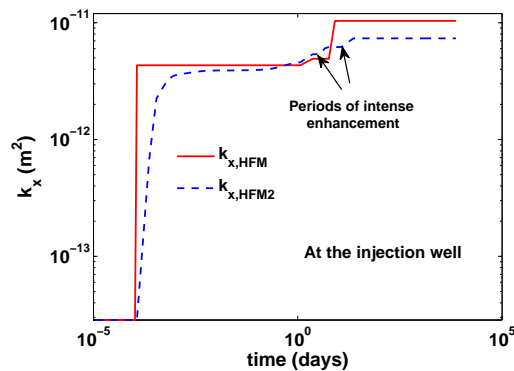
Figure 5.59: Longitudinal permeability k_x history at the injection well: Comparison between the simulations using HFM or HFM2.
