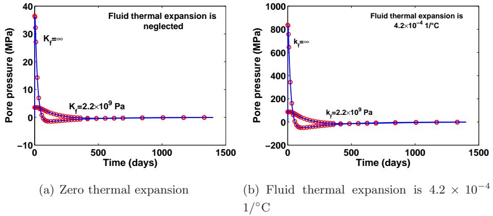
Figure 3.6: Pore pressure time profiles at ( x_2 = 10 m) without and with considering the thermal expansion of pore fluid.
