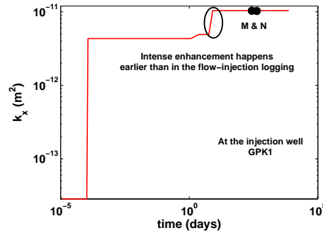
Figure 5.23: Longitudinal permeability k_x history at the injection well GPK1. Points M and N correspond to the period of intense permeability enhancement in figure (5.22). Intense permeability enhancement happens earlier than in the flow-injection logging, figure (5.22).
