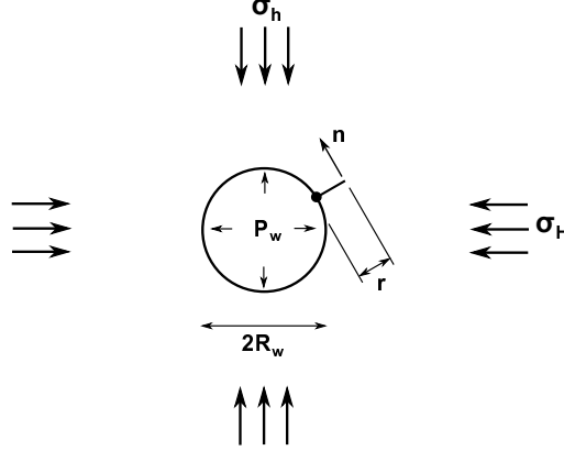
Figure 5.50: Vertical borehole with vertical fracture of average radius r and arbitrary direction \mathbf{n} .
