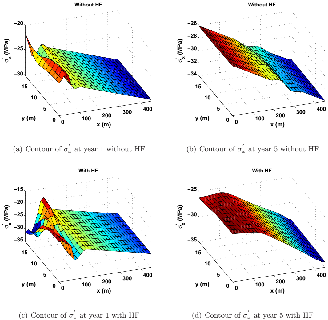
Figure 4.36: Contours of longitudinal effective stress \sigma'_x at two times with/without HF.
