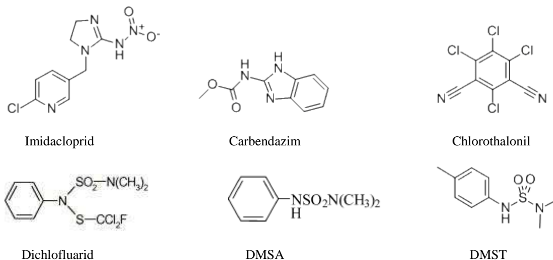
Fig. 3: Structure of pesticides frequently found in coastal areas
