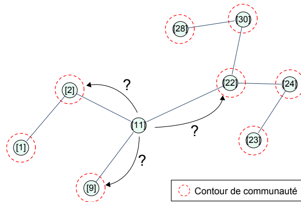
FIGURE 3.2 – Phase itérative
