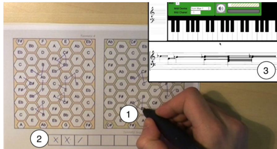
Figure 5.10: Using PaperTonnetz to create and listen to a musical sequence. (1) The user taps on a handwritten path to listen to the corresponding melody and add it to the current track. (2) The sequencer assembles existing paths into tracks. (3) The Max patch displaying the current track made with several paths added as melodies and chords.
