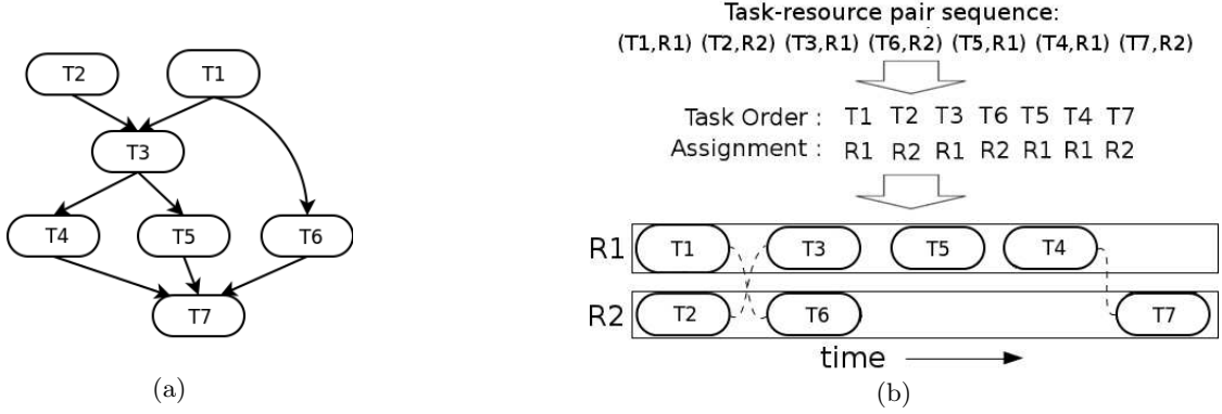
Figure 6.13: Scheduling a job containing 7 interdependent tasks on a grid of 2 resources. Left: The dependency graph of tasks in the job. Right: The illustration of an execution plan.
