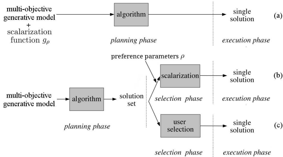
Figure 4.2: The three application scenarios for MORL. (a) Known preference scenario; (b) Varying preference scenario; (c) Decision support scenario (adapted from [Roijsers et al., 2013]).
