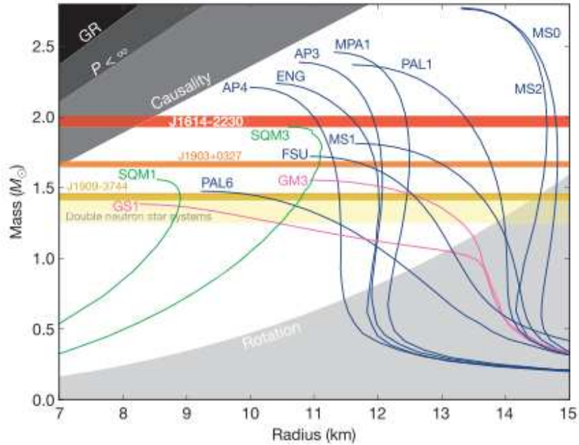
(A) Mass–Radius diagram for typical EOSs
