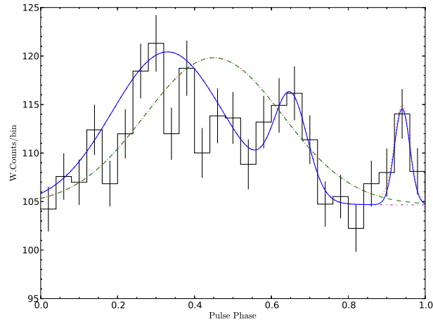
(C) J1913+0904
