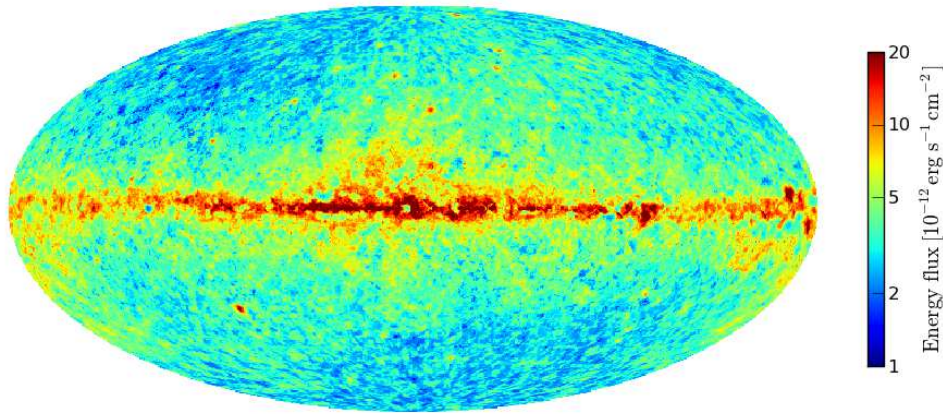
Figure 3.8: Fermi -LAT sensitivity map above 100 MeV with three-year exposure for the P7SOURCE_V6 event class for a point source with pulsar-like exponentially cutoff power law energy spectrum (adapted from 2PC Abdo et al. 2013).
