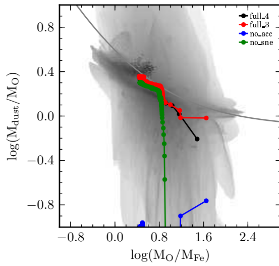
Figure 4.10: Local dust-density weighted diagram for full_4 , in \alpha - \log(M_{\text{dust}}/M_{\odot}) space, at t = 3 Gyr and global diagram inside R < 5 kpc. Grey line is an eye-guide which assumes M_{\text{dust}} \propto M_{\text{O}} + M_{\text{Fe}}
