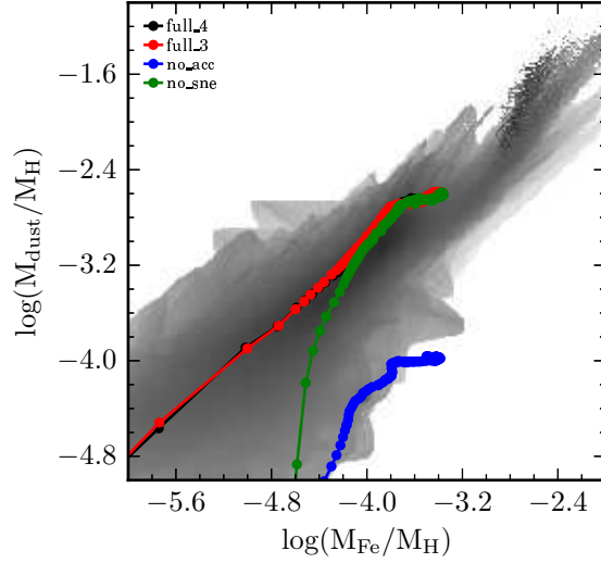
Figure 4.9: Global diagram for the four simulations, inside R < 5 kpc and local diagram for full1.4 at t = 3 Gyr.
