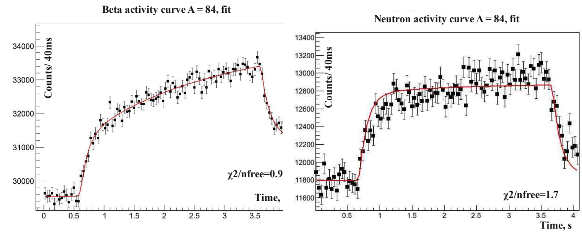
FIGURE 6.32: Reproduced beta (left) and neutron(right) activity curves, A = 84
