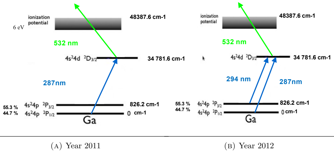
FIGURE 4.5: Laser ionization schemes at ALTO
