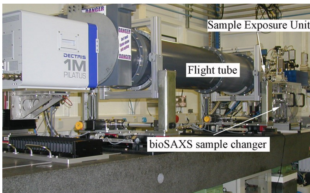
Figure 48 Experimental apparatus of the ID14-3 beamline at the ESRF. The bioSAXS beamline apparatus is indicated in white boxes. Details are described in the text.
