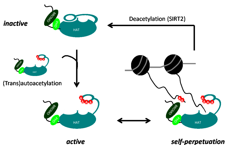
Figure 1 Proposed model for p300/CBP 'core' regulation. Cycles of acetylation/deacetylation events are important for p300/CBP activity, as well as bromo- and PHD- domains. In the figure are shown the bromodomain (bottle green), the PHD domain (apple green) and the HAT domain (navy green). Acetylated lysines are indicated by red hexagons. Nucleosomes: black circles; histone tail: black line; DNA: gray line.
