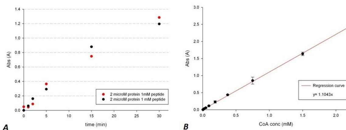
Figure 42 HAT assay time course and CoASH standardization. (A) A time course of the H3 peptide acetylation by p300 HAT \Delta 1520-1580 using a colorimetric DTNB coupled assay. Absorbance at 412 nm is plotted as a function of the time (min). The experiment was done in duplicate (red and black dots) at 30°C. (B) The standard curve calculated using serial dilution of CoASH. Absorbance at 412 nm due to the formation of thiophenolate from the DTNB reaction is plotted as a function of the CoASH concentration (mM). Experiments were carried out at 30°C and the reaction was stopped after 15 minutes.
