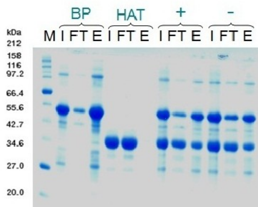
Figure 40 GST-pull-down using GST-BP and HAT \Delta loop/Y1467F. SDS-PAGE gel showing a pull-down in presence (+) or absence (-) of a BP substrate (histone H3 peptide K14K18 diacetylated). The molecular weight (kDa) of the marker is given. Negative controls of the GST-BP and of the HAT domain alone are also shown (names are indicated above the gel). M, marker; I, input; FT, flow through; E, elution. Proteins are visualized by Coomassie blue staining.
