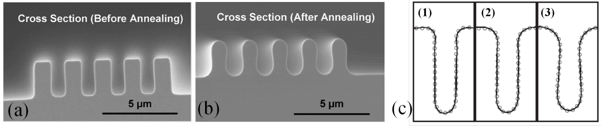
Fig. 3.2: Cross sectional SEM micro-graphs of Si trenches, (a) before and (b) after hydrogen annealing at 1100 °C and 10 Torr for 5 min [17]. (c) Calculated trench profiles (solid curves) are compared with experimental profiles (open circles) extracted from SEM images. Trenches were annealed in H_2 at 1000 °C for (1) 30 s, (2) 180 s, and (3) 600 s [13].
