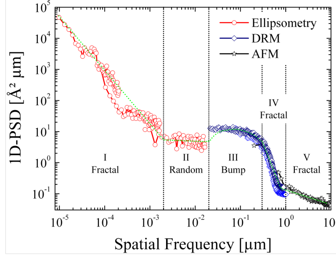
Fig. 1.35: PSD_{1D} function representing the top silicon layer thickness variations, measured by: (left) Ellipsometry (three different sampling periods: \Delta x_1 = 30 \mu m , \Delta x_2 = 300 \mu m and \Delta x_3 = 2420 \mu m . (center) Differential Reflectivity Microscopy (image size: 66.6 \times 88.6 \mu m^2 ) and (right) AFM (scan-size: 30 \times 30 \mu m^2 and 10 \times 10 \mu m^2 ).
