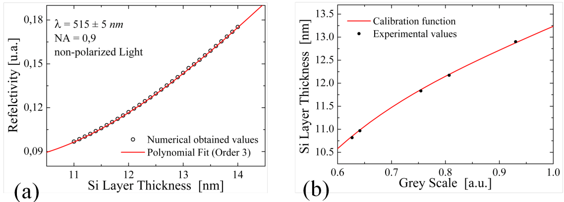
Fig. 1.27: (a) Reflectivity coefficient evolution as a function of the top silicon layer thickness using the optimal wavelength. (b) Calibration curve (red line) obtained from experimental values of 5 SOI wafers ( Si layer thickness measured by SE . Grey scale obtained by DRM).
