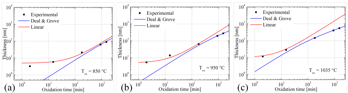
Fig. 4.2: Comparison between thicknesses measured by ellipsometry (points), and that obtained from Deal and Grove model (blue line). Dry oxidation has been performed using mirror-polished Si wafers.
