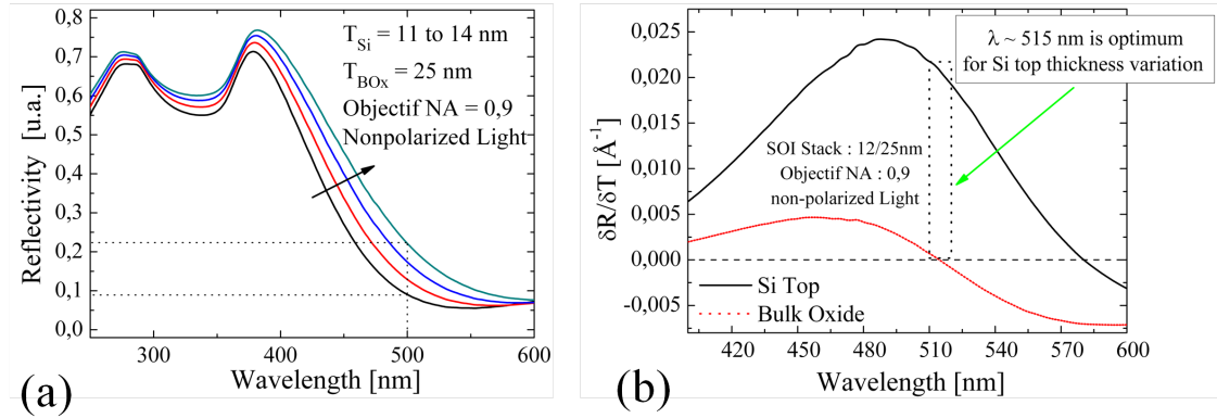
Fig. 1.26: (a) Reflectivity variations for different top silicon layer thicknesses. (b) Sensitivity values obtained for a thickness variation of 1 Å of the top silicon layer (black line) and of the BOx.
