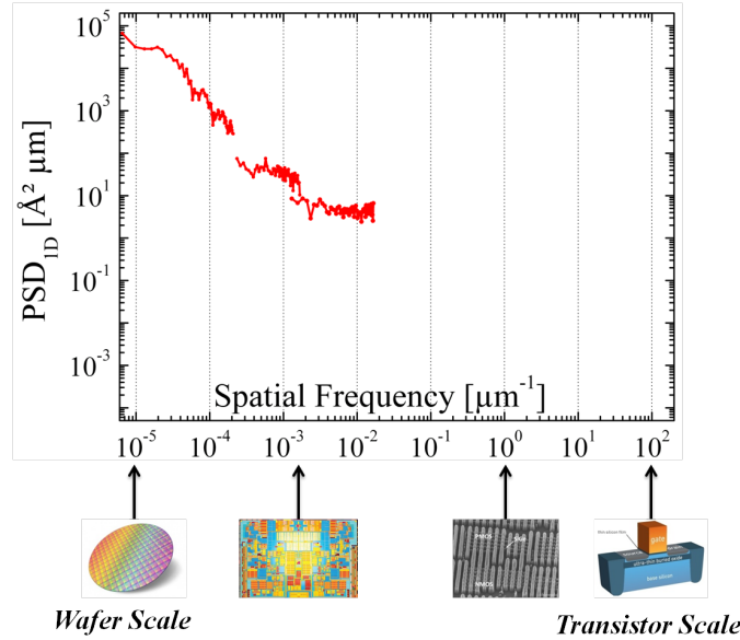
Fig. 1.21: Corrected PSD_{1D} functions describing thickness variation of the silicon top layer of a SOI wafer measured by SE. Sampling period used for these measurements are \Delta x_1 = 30 \mu m , \Delta x_2 = 300 \mu m and \Delta x_3 = 2420 \mu m .
