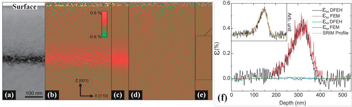
Fig. 2.5: Dark-field electron holography of a (001) Si crystal implanted at 10^{16} \text{ H}^+ \text{ cm}^{-2} . (a) Conventional bright-field TEM image under two-beam condition for the (111) diffracted beam; (b) out-of-plane \varepsilon_{zz} and (d) in-plane \varepsilon_{xx} strain maps obtained by DFEH ; (c) and (e) the corresponding strain components calculated from a FEM model. (f) Vertical strain profiles of the two components of \varepsilon_{zz} and \varepsilon_{xx} , extracted from the experimental and simulated images. Zero depth corresponds to the surface of the sample. The inset compares the H depth distribution (by SRIM ) and the strain profile (by DFEH ). (adapted from [5]).
