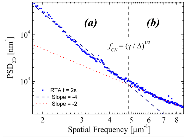
Fig. 3.9: High frequency range of the PSD_{2D} function of annealed surfaces (2 s at 1200 °C). Two scaling regimes are evidenced, separated by a characteristic frequency ( f_{CN} ).
