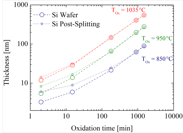
Fig. 4.4: \text{SiO}_2 thickness for dry oxidation of \text{Si} wafers with mirror-polished (circles) and post-splitting-like (stars) initial surfaces.
