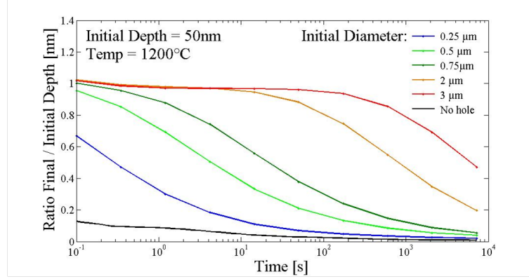
Fig. 3.22: Evolution of the ratio of final/initial depth of shallow holes during thermal annealing at 1200 °C for different initial diameters.
