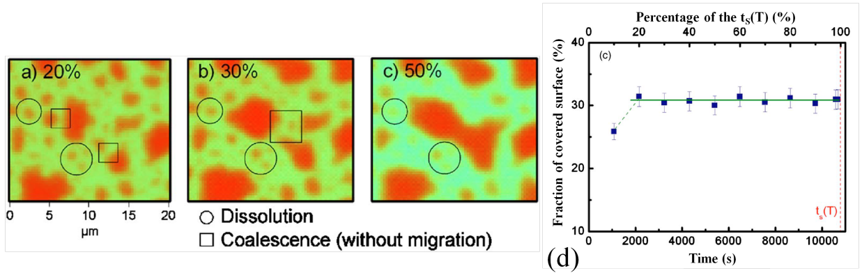
Fig. 2.15: Optical microscope images of buried micro-cracks after an annealing at 350 °C for 20% (a), 30% (b), and 50% (c) of t_s(T) . The images illustrate the Ostwald ripening and the coalescence mechanisms. (d) Time dependence of the fraction of surface covered by micro-cracks [23].
