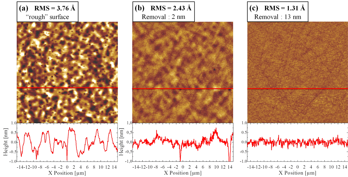
Fig. 5.10: Typical AFM Images ( 30 \times 30 \mu m^2 ; 512 \times 512 pixels) of annealed post-splitting SOI wafers («rough» surface) before (a) and after CMP process using slurry 1. Images shown correspond to the minimal (2 nm) (b) and the maximal (13 nm) material removal.
