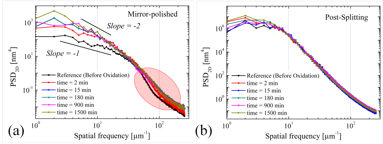
Fig. 4.10: PSD_{2D} functions describing the topography evolution of Si wafers during dry oxidation at 850^\circ\text{C} for (a) smooth and (b) rough initial surfaces.
