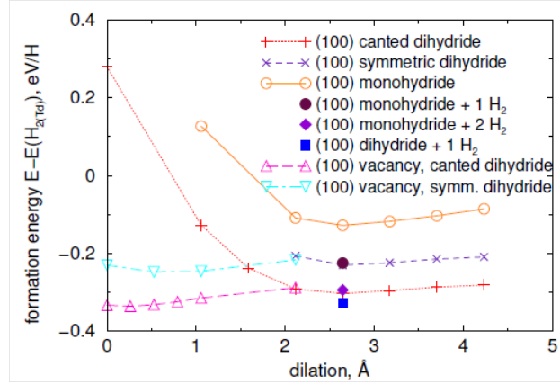
Fig. 2.9: Energies of hydrogenated Si(100) internal surfaces as a function of dilatation with the monohydride ( Si-H ) and symmetric and canted dihydride ( Si-H_2 ) structures. (adapted from [32]).
