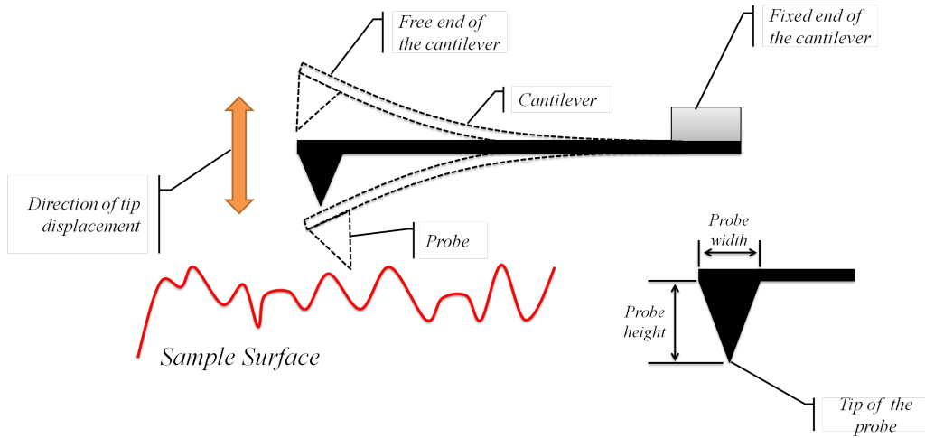
Fig. 1.8: Schematic of the atomic force microscopy.
