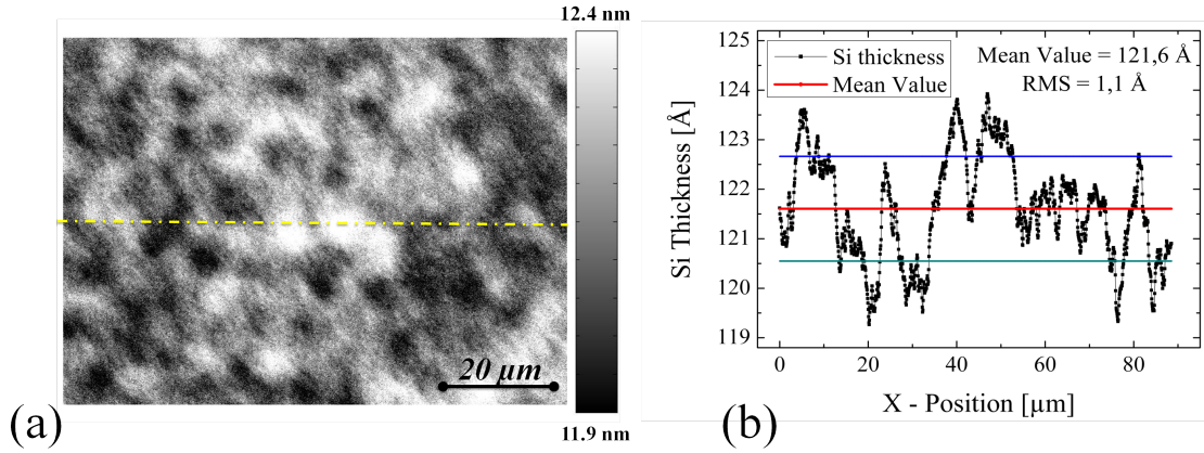
Fig. 1.28: DRM image obtained with a Zeiss Axiotron 2 microscope with a 100 \times magnification objective ( NA = 0.9 ), using a green interferometric filter (515 nm) and a CCD camera (1292 \times 968 pixels). (a) 88.6 \times 66.6 \mu m^2 image where the grey level of each pixel represents the thickness of the top silicon layer. (b) Thickness profile obtained from the image shown in a).
