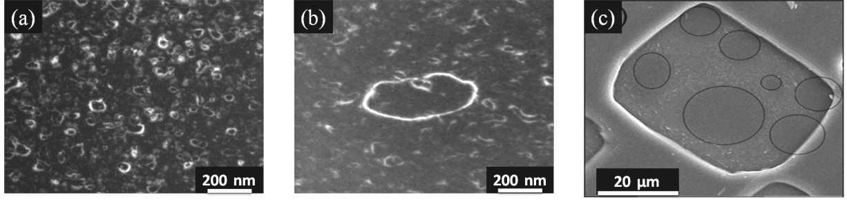
Fig. 2.14: Plane view TEM images of implanted and annealed Si samples at 360 °C during (a) 11 min where only platelets can be observed, and (b) 67 min showing a micro-crack [24]. (c) High-magnification SEM micrographs showing the exfoliation morphologies for implanted and annealed Si samples (the dashed circles highlight the circular feature observed in the bottom of the exfoliated region. (adapted from [40]).
