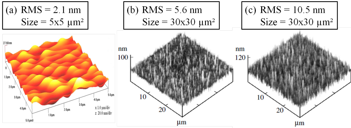
Fig. 2.21: AFM images of post-splitting surfaces obtained from: (a) post-splitting wafer with B-H co-implantation (adapted from [49]). (b) from a wafer containing a buried doped layer and (c) from a wafer without buried layer. (adapted from [50])
