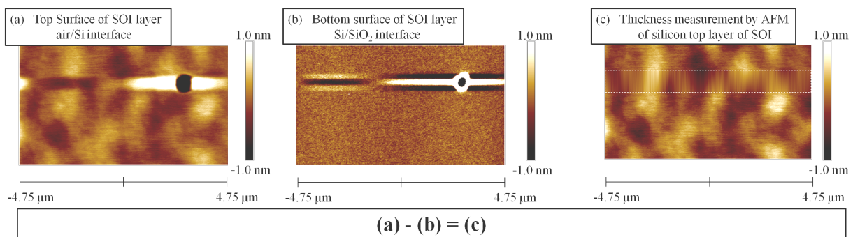
Fig. 1.24: AFM images obtained after resizing and centring of interfaces of the top silicon layer: (a) top and (b) bottom interface. (c) thickness variations image obtained by subtraction of height values.
