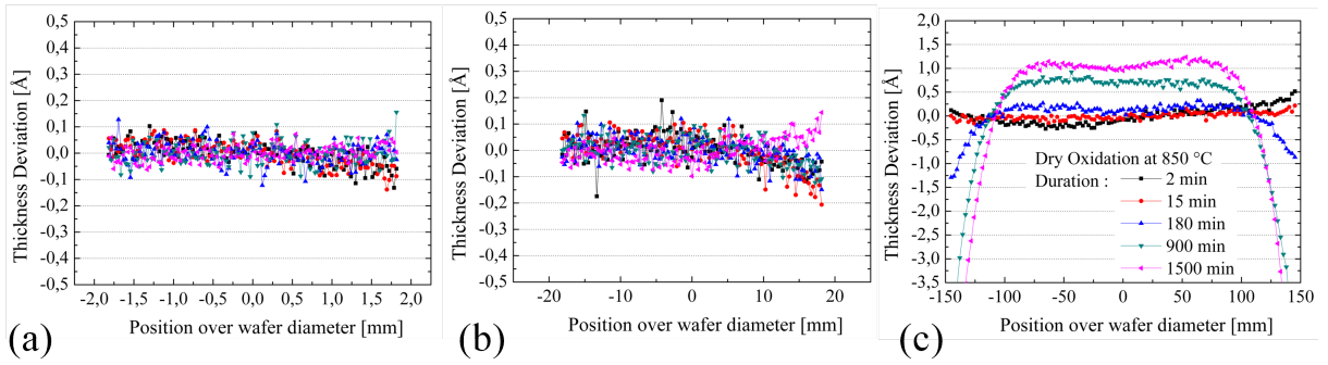
Fig. 4.5: Thickness of oxide layers for dry oxidation measured by SE using three different sampling periods: (a) \Delta x_1 = 30 \mu\text{m} , (b) \Delta x_2 = 300 \mu\text{m} and (c) \Delta x_3 = 2420 \mu\text{m} .
