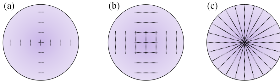
Fig. 1.14: Schematic illustrations showing the location, across the wafer, of points composing profiles for thickness measurements using three different sampling periods (a) \Delta x_1 = 30 \mu m , (b) \Delta x_2 = 300 \mu m and (c) \Delta x_3 = 2420 \mu m .
