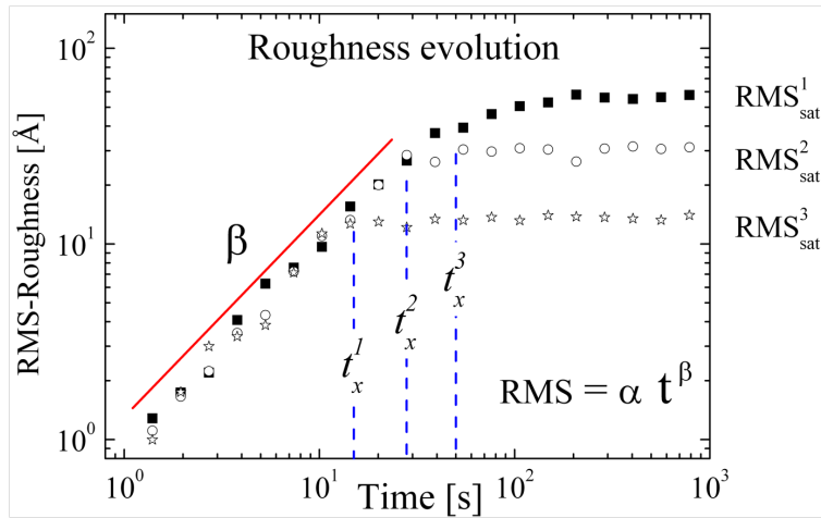
Fig. 1.4: Evolution of the RMS value with time in the case of ballistic growth of a interface. One observe two regimes: (a) increase following a power law (straight line in log-log plot) and (b) a saturation after t_x^i .
