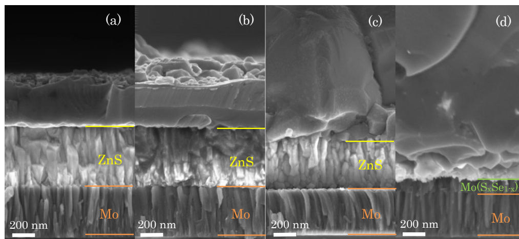
Figure 36: SEM images showing the formation of CZTSSe at different steps in the selenization process of Stack A: (a) after selenization at 350°C, (b) after selenization at 450°C, (c) after selenization at 570°C, (d) after selenization at 570°C with a 30 minute thermal plateau
