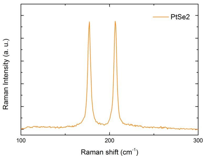
Figure 65: Raman spectrum of \text{PtSe}_2 .
