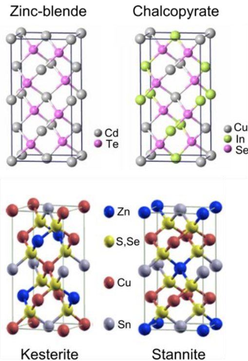
Figure 16: Crystal structure representation of binary, ternary and quaternary compounds.
