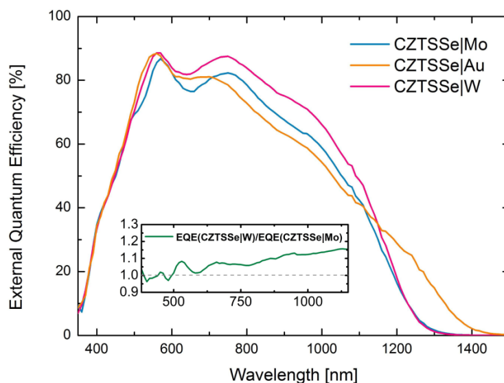
Figure 71: External quantum efficiency measurements on best performing CZTSSe solar cells with Mo-, Au-, W-back contacts. Bandgaps E_g are deduced via linear extrapolation of the low energy slope of the EQE. The inset shows EQE spectrum of CZTSSe|W solar cell divided by the EQE spectrum of CZTSSe|Mo solar cell.
