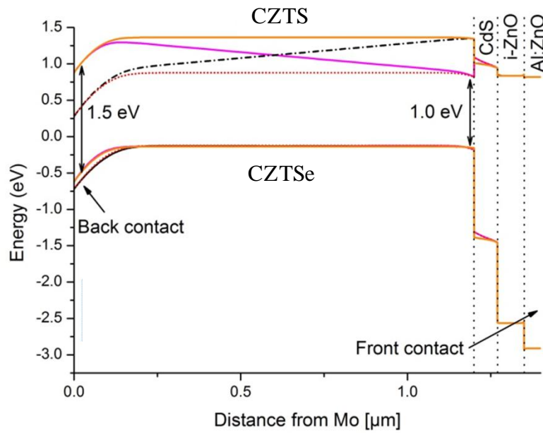
Figure 80: Graphical representation of the band alignments within different CZTSSe solar cells in the dark: CZTS (orange line), CZTSSe (red dotted line), bandgap decreasing from Mo to CdS (purple line), bandgap decreasing from CdS to Mo (black line).
