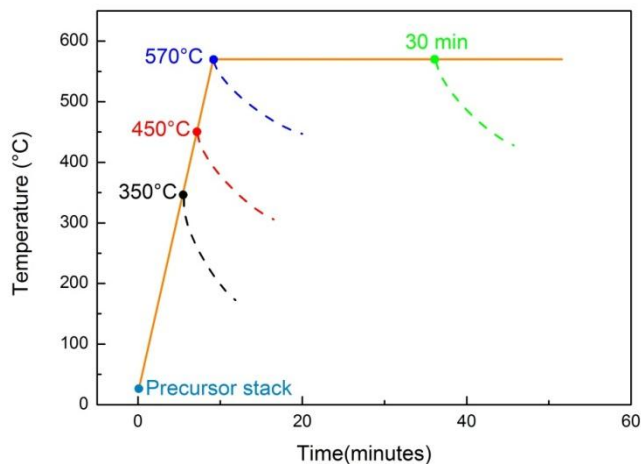
Figure 35: Temperature profiles of the samples which underwent selenization at 350°C, 450°C and 570°C (with and without the thermal plateau).
