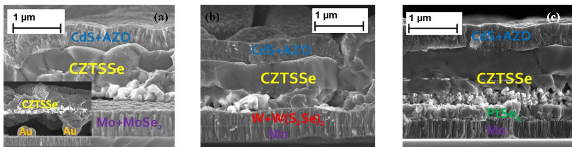
Figure 67: SEM images of Al:ZnO/i-ZnO/CdS/CZTSSe/BC/Mo solar cells synthesized on Au (CZTSSe|Au) (a), W (CZTSSe|W) (b), Pt (CZTSSe|Pt) (c). The inset in Fig. 64a shows the SEM image of gold particles after selenization process.
