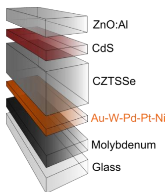
Figure 68: Schematic of Al:ZnO/i-ZnO/CdS/CZTSSe/BC/Mo solar cells.
