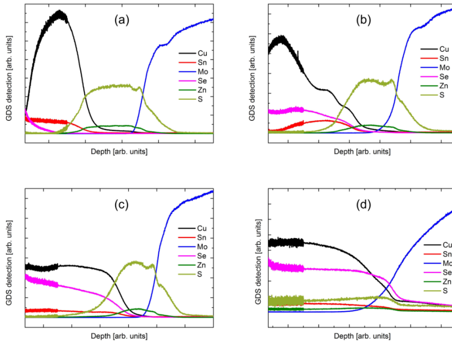
Figure 43: GDS spectra of Stack B: (a) 350°C, (b) 450°C, (c) 570°C, (d) 570°C - 30min
