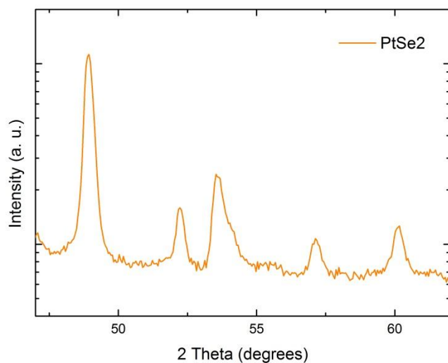
Figure 64: XRD patterns of \text{PtSe}_2 .
