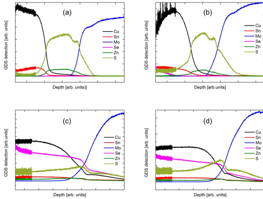
Figure 42: GDS spectra of Stack A: (a) 350°C, (b) 450°C, (c) 570°C, (d) 570°C - 30min
