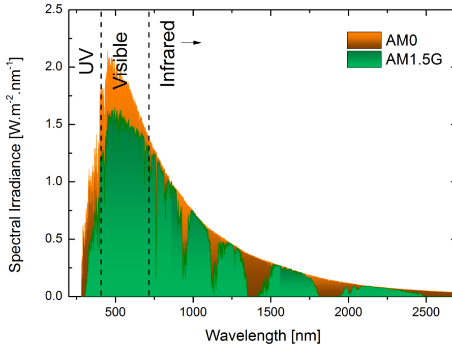
Figure 2: Solar irradiance spectrum above atmosphere and at Earth surface.
