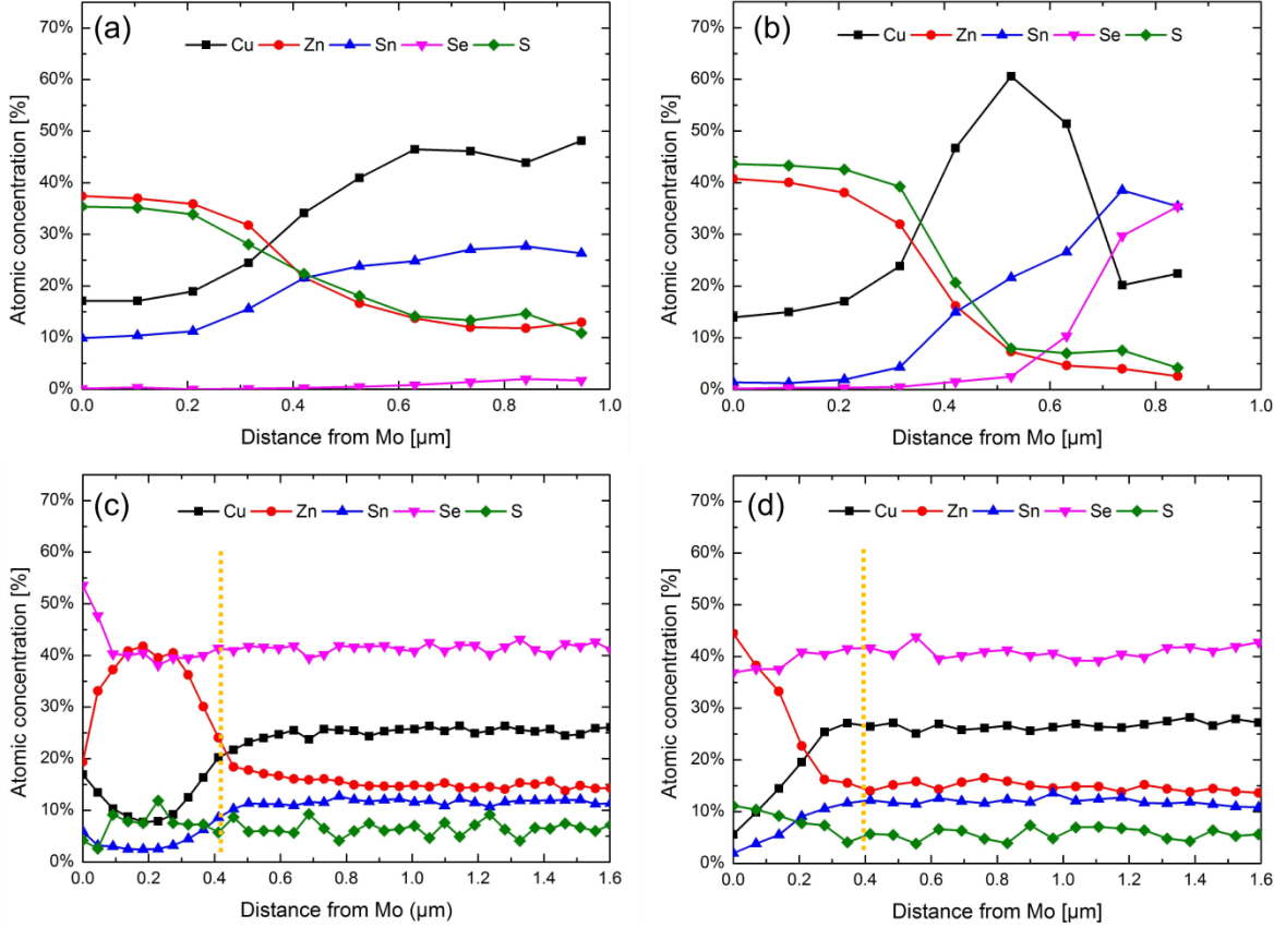
Figure 38: Cross-section EDS profiles of stack A selenized at 350°C (a) and 570°C – 30min (c); cross-section EDS profiles of stack B selenized at 350°C (b) and 570°C – 30min (d). All statistical errors are twice the confidence limit. The yellow line in each image is the starting point for the calculation of [Zn]/[Sn] , [Cu]/([Zn]+[Sn]) and [S]/([S]+[Se]) ratios shown in Table 2. The Zn-rich phase on the left of the black line is discarded in the composition calculations
