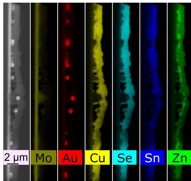
Figure 73: Cross-sectional EDX analysis of CZTSSe|Au performed in a TEM.
