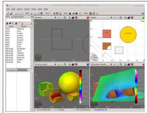
(b) Facilitated editing of the FLUKA geometry using FLAIR [21].
