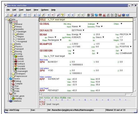
(a) Facilitated editing of the FLUKA input using FLAIR [21].
