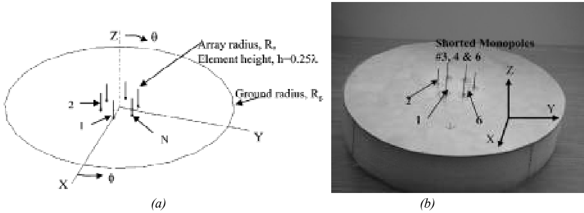
Figure 3.7 – Wire circular monopole array (CMA). (a) Geometry of an N - element CMA on a finite ground plane fed using a SMA probe. Its parameters are: R_a = 0.25\lambda and R_g = 1.50\lambda . (b) Photograph of 6 -element CMA designed for 2.8 GHz, the R_g = 1.40\lambda = 15 cm, h = 0.25\lambda = 2.65 cm, R_a = 0.234\lambda = 2.5 cm, and the inter-element angle is 60^\circ [25].
