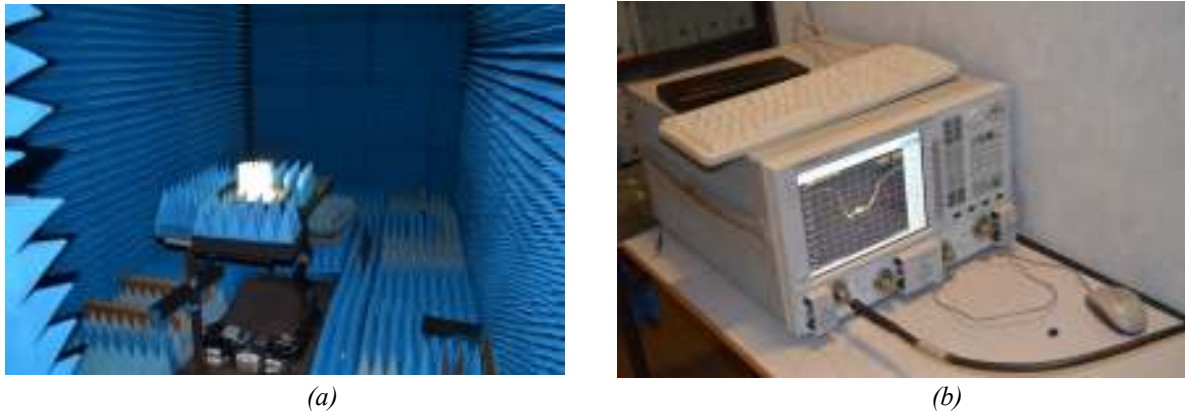
Figure 3.48 – Antenna input impedance measurement apparatus. (a) RRA with activated elements. (b) Vector network analyzer (Agilent N5242A).
