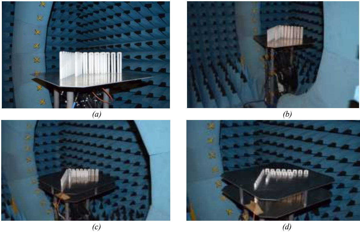
Figure 3.82 – Photograph of the fabricated CRA with primary and secondary ground plane. (a)-(b) The h is 115 mm. (c) The h is 54 mm with the inserted secondary ground plane. (d) The h is 15 mm with the inserted secondary ground plane.
