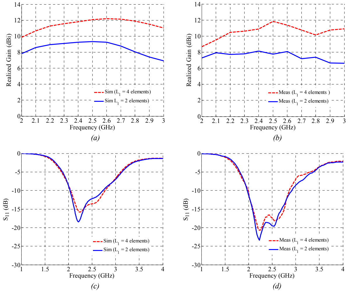
Figure 3.96 – Performances of corner reflector antenna (CRA1) at 2.4 GHz. (a) Simulated realized gains. (b) Measured realized gains. (c) Magnitude of simulated reflection coefficients, S_{11} . (d) Magnitude of measured reflection coefficients, S_{11} .
