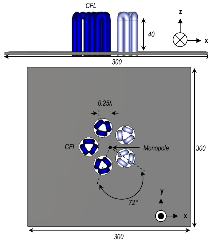
Figure 3.35 – Round reflector antenna using Triple Bias CFL consist of 5 elements. Only three elements are activated at the same time to reflect beam in forward direction. (Units in mm)
