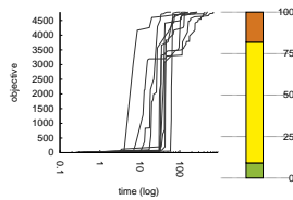
1.146 mario_mario_t_hard_1 with PGLNS
