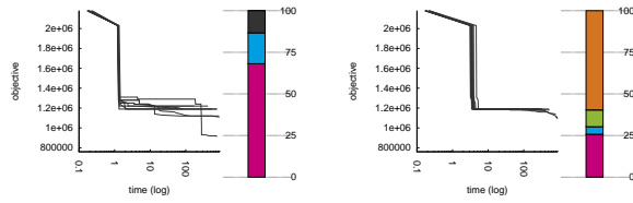
1.74 league_model190-18-20 with EBLNS 1.75 league_model190-18-20 with PaEGLNS
