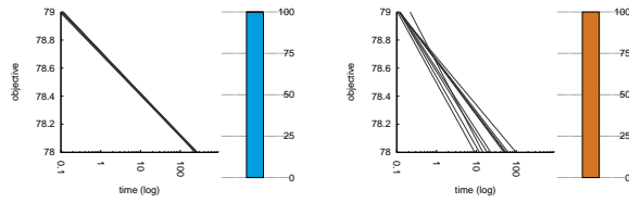
1.94 rcpsp_13 with EBLNS with 1.95 rcpsp_13 with PaE-GLNS
