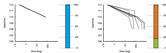
1.19 cars_cars_41_66 with EBLNS 1.20 cars_cars_41_66 with PaEGLNS
