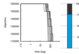
1.67 league_model155-3-12 with cftLNS
