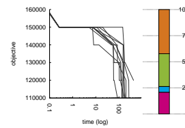
1.70 league_model155-3-12 with PaEGLNS
