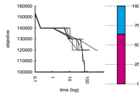
1.64 league_model150-4-4 with EBLNS
