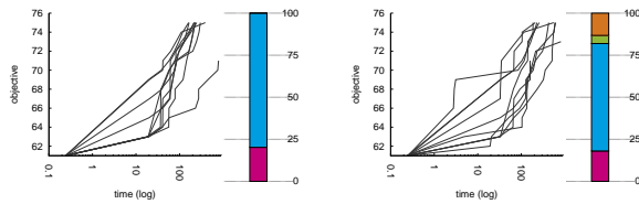
1.239 still-life_12 with EBLNS 1.240 still-life_12 with PaEGLNS
