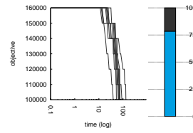
1.62 league_model150-4-4 with cftLNS
