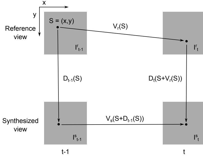
Figure 7.3: Epipolar constraint
