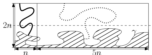
Figure 9: An event implying the occurrence of \mathcal{A}(e, \gamma) and \mathcal{A}^*(e^*, \gamma) for the same edge e in \gamma .
