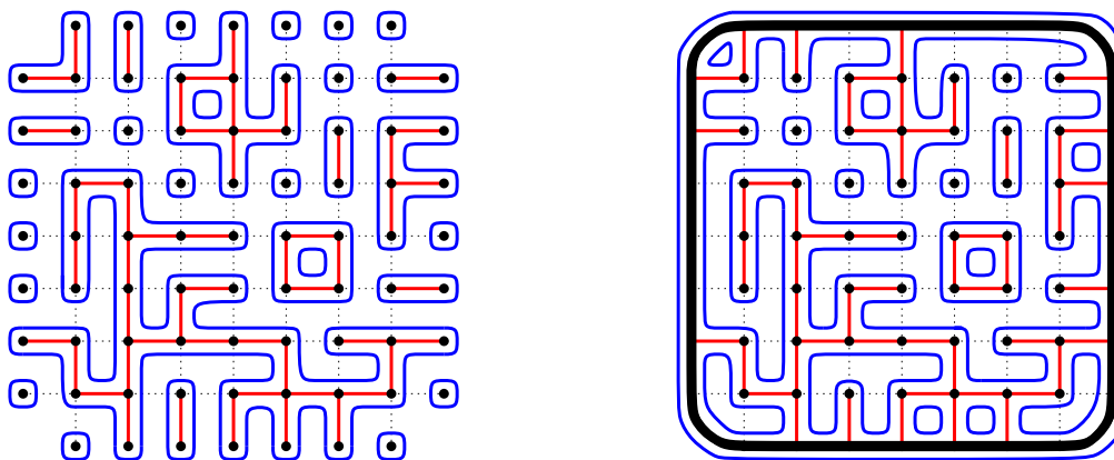
Figure 14: The bond-clusters defined by the configuration on \Lambda_n (left) and \tilde{\Lambda}_n (right). There are k_0(\omega) bond-clusters on the left, k_1(\omega) on the right.
