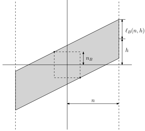
Figure 7.3: Definition of \ell_B(n, h)
