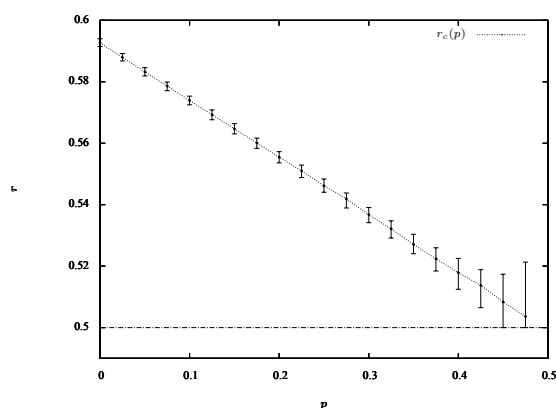
Figure 10: Simulation results for different values of p < p_c^L . The dashed line was obtained via a non-rigorous correction method.
