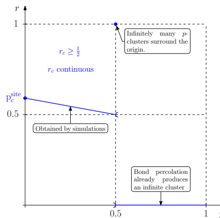
Figure 11: Expected behavior for r_c on the square lattice.
