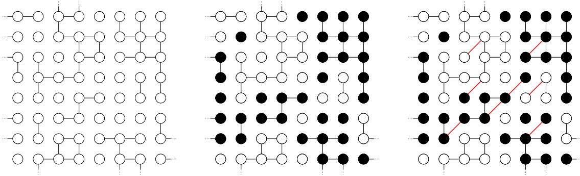
Step 1: Bernoulli bond percolation.
