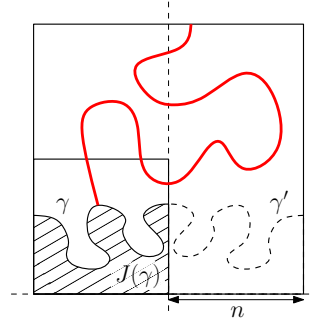
Figure 3: The event \mathcal{V}_\gamma
