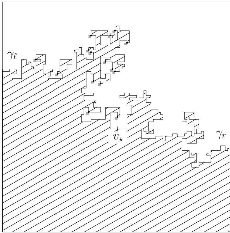
Figure 3.14: The set of exposed points (represented by black squared dots) and their associated exposed boxes (grey squares).
