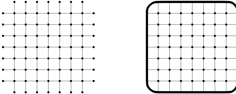
Figure 13: The graphs \Lambda_n (left) and \tilde{\Lambda}_n (right). On the right, the thickened boundary represents a single vertex.
