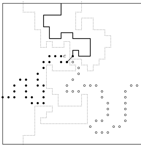
Figure 3.7: The event \mathcal{A}_{\text{mixed}}(e)
