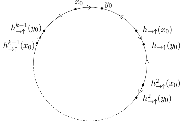
FIGURE 3.5. Dynamics of an element of H
