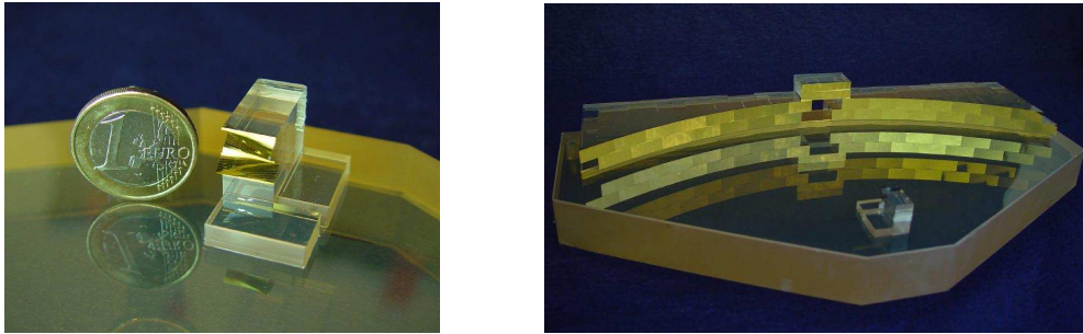
Figure 2.3: The actual image slicer ( left ) that cuts the image in 32 slices, and set of mirrors of SINFONI ( right ) that arrange these slices along a 'pseudo-longslit'.
