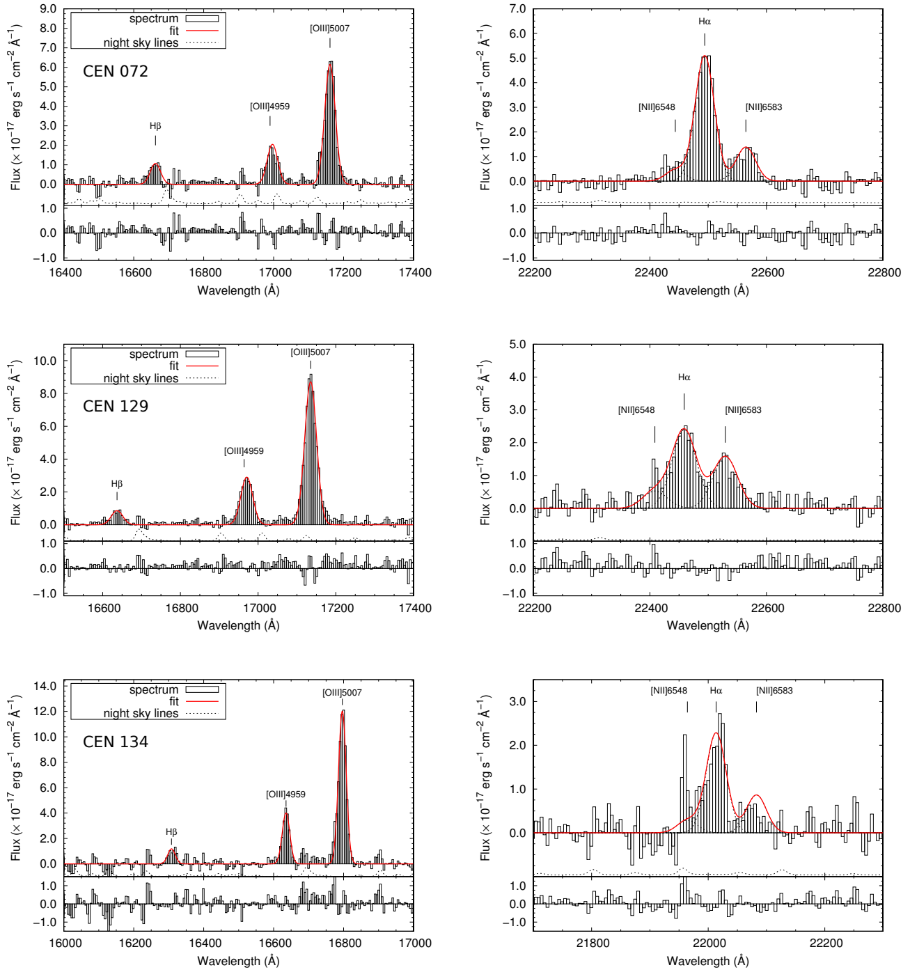
Figure 4.13: Spectra of the CENSORS sample, integrated over pixels where the [OIII] emission line is detected at \text{SNR} > 5 . The left column show spectra centered on the H \beta and [OIII] doublet emission lines and the right column is centered on the H \alpha + [NII] complex. All lines are well fitted by single Gaussians, which parameters can be found in Table 4.16, 4.17 and 4.18. Residuals to the fit are shown in the bottom panel.
