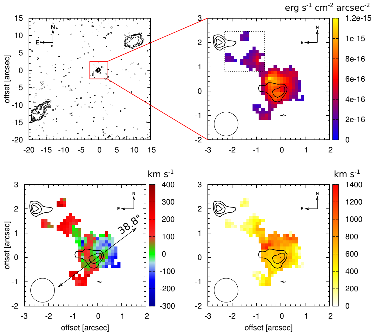
Figure 5.4: Radio observations of TXS 2355–003 at 5.0 GHz (top left) with the field of view of SINFONI in red ; and H\alpha surface brightness (top right), velocity (bottom left) and velocity dispersion (bottom right) from our SINFONI observations.
