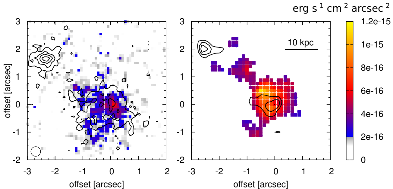
Figure 5.11: Left : NB image of TXS 2355–003, from which the scaled contribution of broad-band image is subtracted. This image therefore represents the contribution of the H\alpha + [NII] emitting gas. Right : H\alpha surface brightness of TXS 2355–003, as derived from our SINFONI observations. The scale is the same in both images and the solid contour lines represent the continuum.
