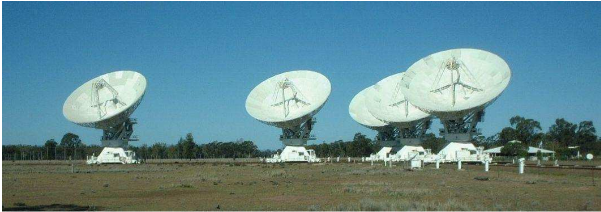
Figure 2.8: View of 5 of the 6 antennas forming the ATCA, in a compact configuration: the three antennas on the right are on the East-West tracks while the the two on the left are on the North-South track.
